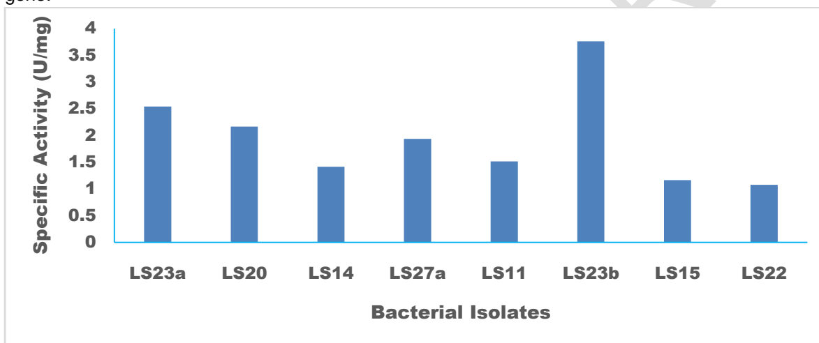
Fig. 1. Secondary screening for protease production by bacterial isolates
