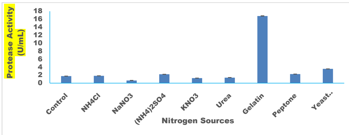
Fig. 7. Influence of nitrogen sources on protease production
