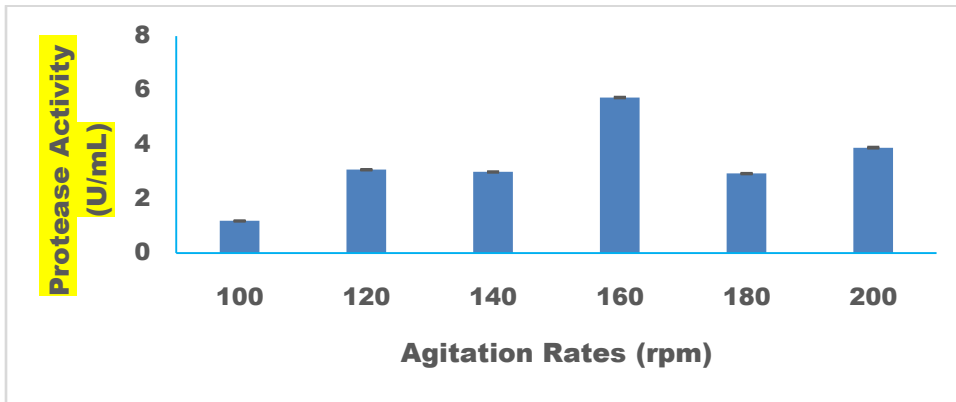
Fig. 9. Influence of agitation rates on protease production
