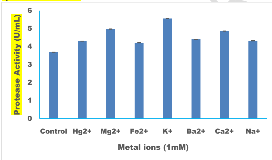
Fig. 10. Influence of metal ions on protease production
