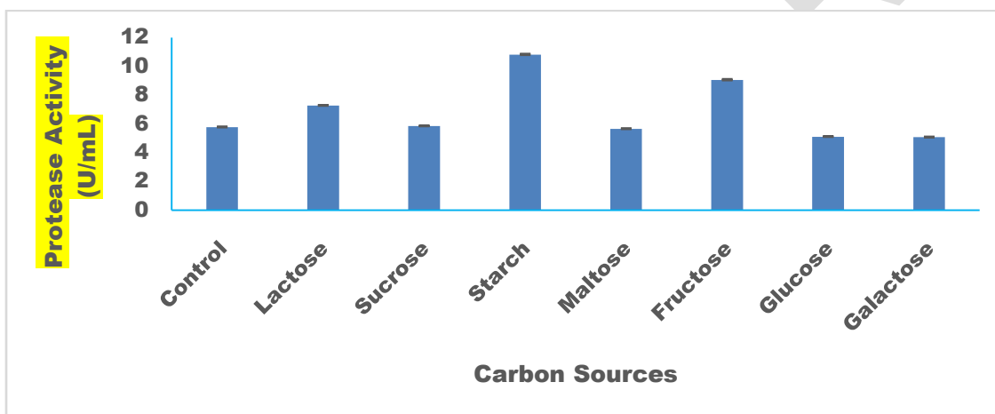
Fig. 6. Influence of carbon source on protease production
