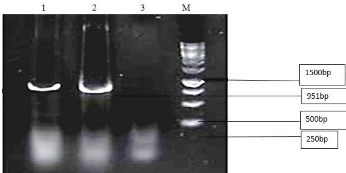
Fig. 2. PCR Amplification of protease ( npr ) gene primer of LS23B. Key: 1: Positive control; 2: Isolate LS23B; 3: Negative control; M: Molecular marker.
