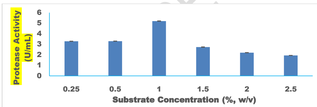
Fig. 8. Influence of substrate concentration (% w/v) protease production
