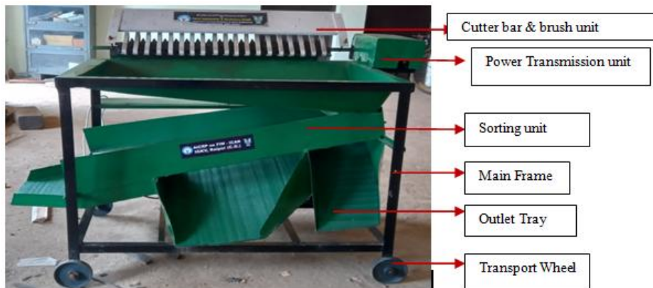
Fig.1 : Developed onion stem and root cutter cum sorting machine
