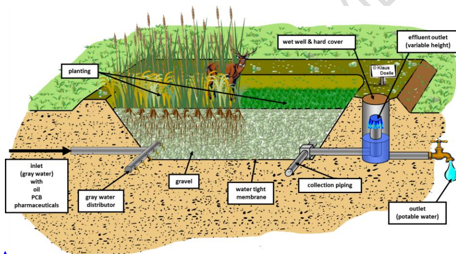
Fig 5: Scetch of a Subterranean Flow Constructed Wetland [22]
