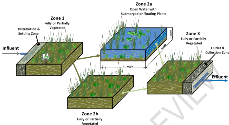
Fig 3: Surface- and Subterranean Flow Constructed Wetland Types [26]
