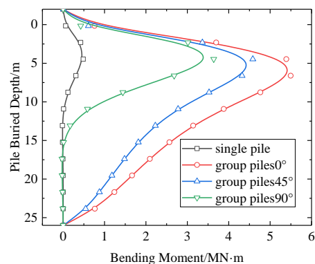
Fig.10 Bending moment distribution curve of pile body
