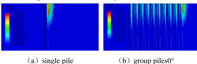
Fig.5 Cloud Chart of Principal Stress Distribution
