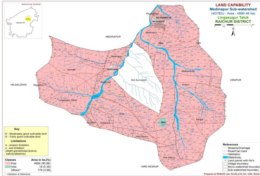
Fig. 5 Land capability classes of MedinapurSub-watershed
