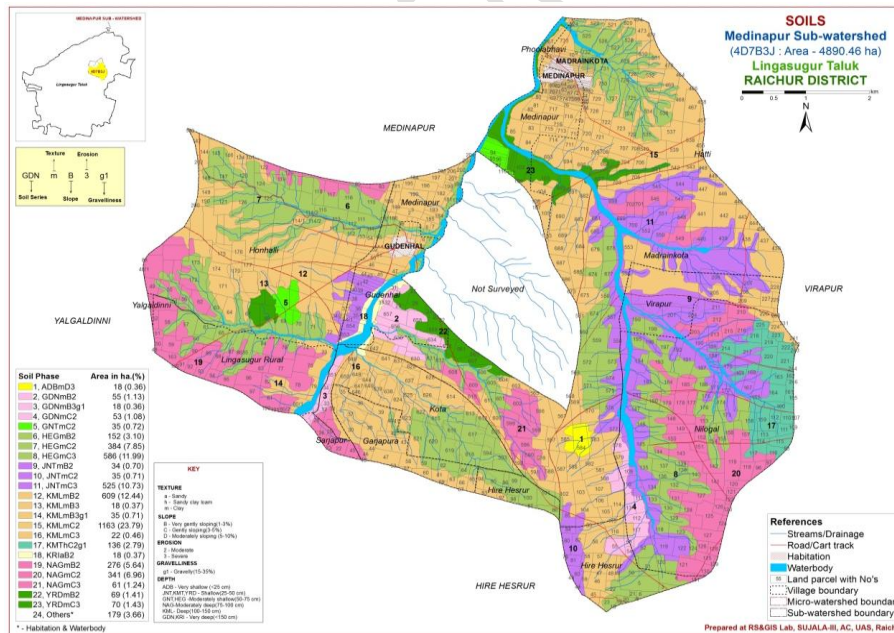
Fig. 4 Soil map of MedinapurSub-watershed
