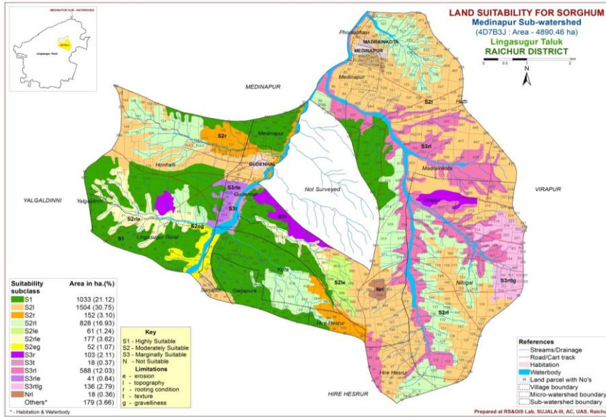
Fig. 11 Land suitability map for Sorghum in Medinapur sub-watershed
