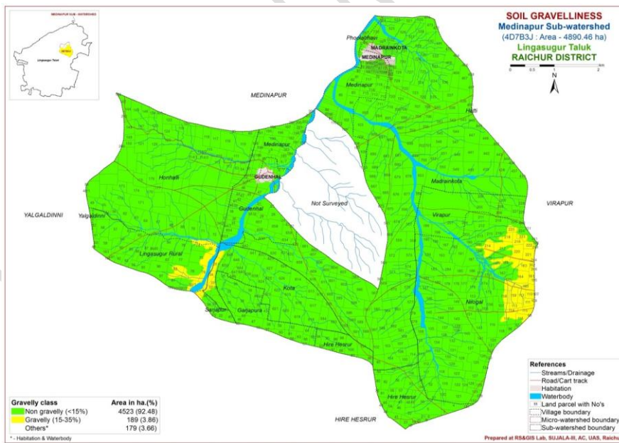
Fig. 8 Soil gravel classes of MedinapurSub-watershed
