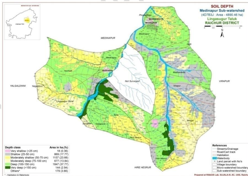
Fig. 6 Soil depth classes of MedinapurSub-watershed
