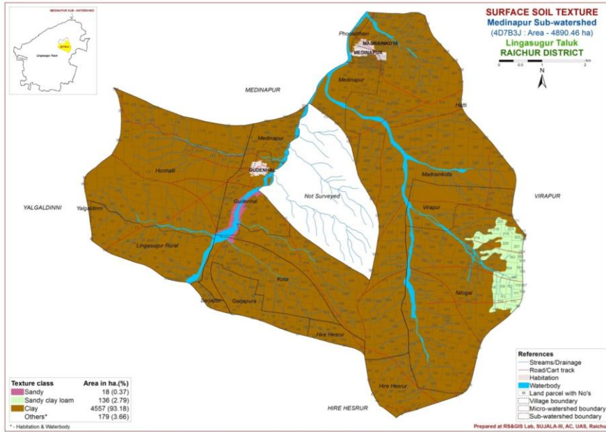
Fig.7 Surface soil texture classes of MedinapurSub-watershed
