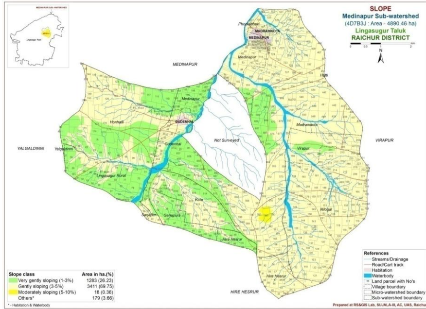
Fig. 9 Slope classes of MedinapurSub-watershed
