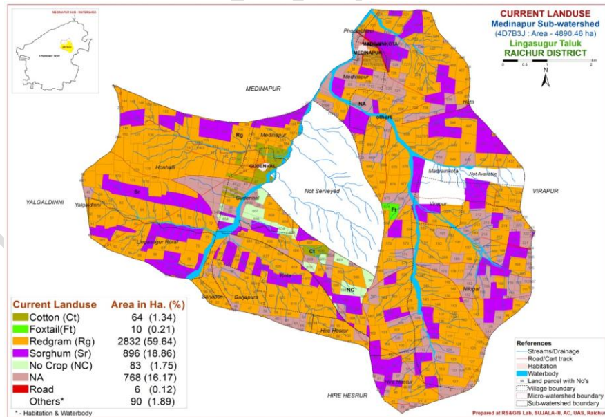
Fig. 10 Current land use of MedinapurSub-watershed
