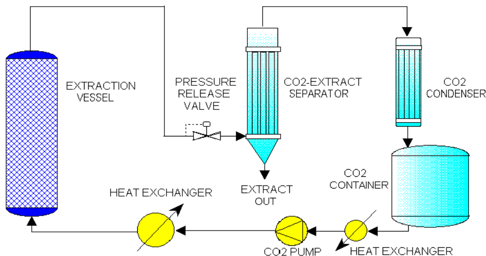
Figure 2: Operating principle of semi batch Supercritical fluid extraction (Source: ResearchGate, 2000)
