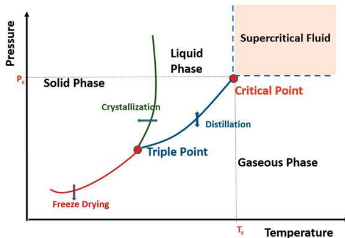
Figure 1: Phase Diagram of Supercritical Fluid (Source: Intechopen, 2022)
