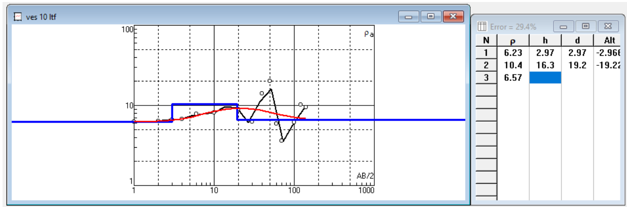
Figure 15: VES station 10 showing graph of apparent resistivity against electrode spacing.
