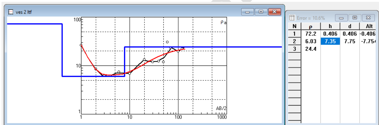
Fig.7:VES Station 2 showing graph of apparent resistivity against electrode spacing.
