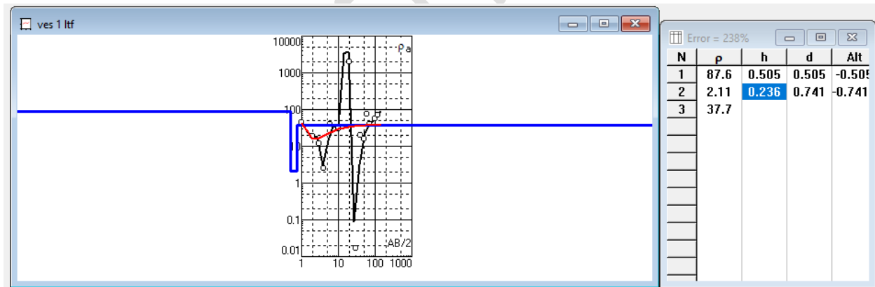
Fig.6: VES Station 1 showing graph of apparent resistivity against electrode spacing.
