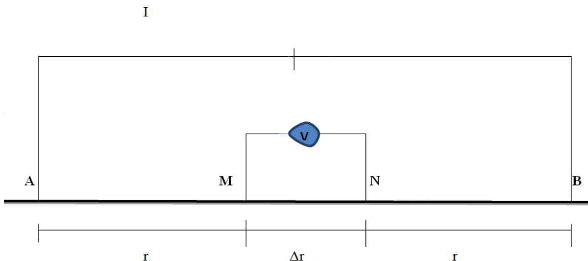
Fig4: Configuration of Schlumberger Array
