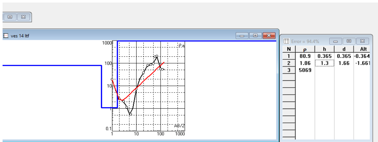
Figure 19: VES station 14 showing graph of apparent resistivity against electrode spacing.
