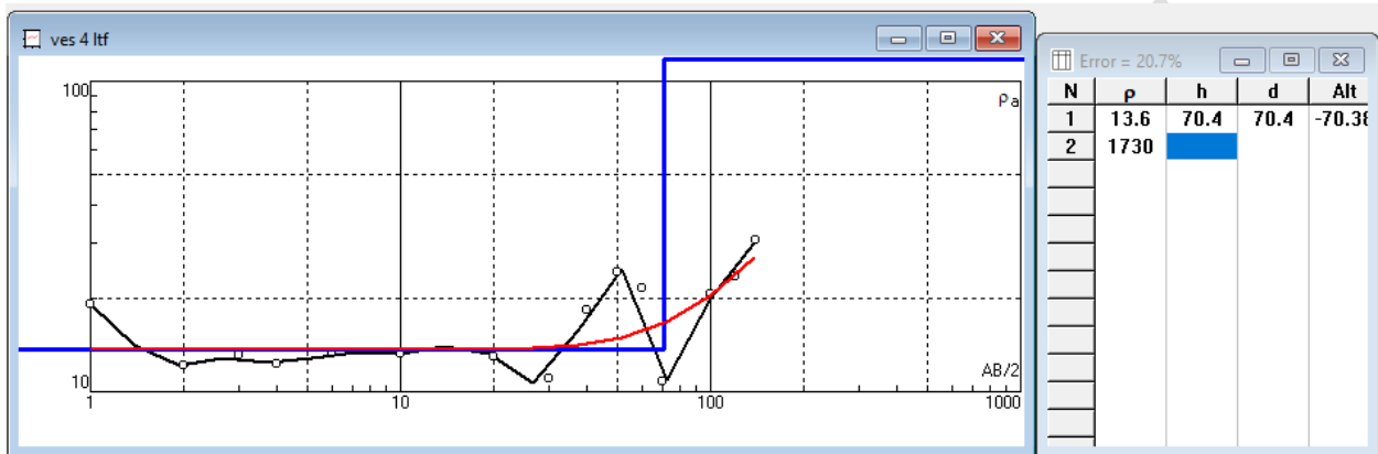
Fig.9:VES station 4 showing graph of apparent resistivity against electrode spacing.
