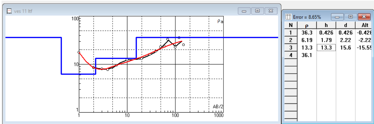
Fig.16: VES station 11 showing graph of apparent resistivity against electrode spacing.
