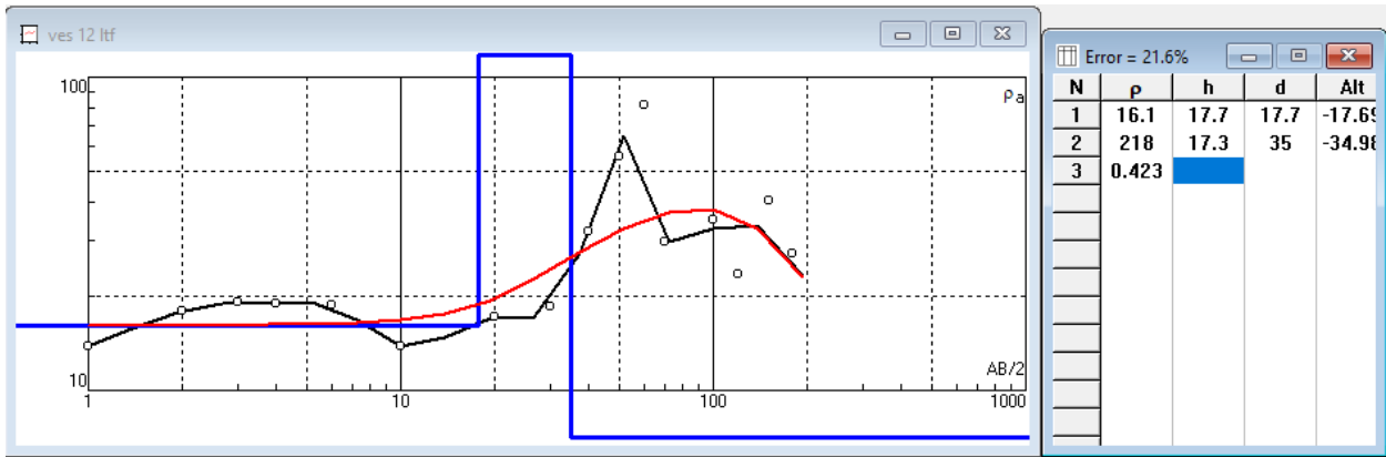
Figure 17: VES station 12 showing graph of apparent resistivity against electrode spacing.
