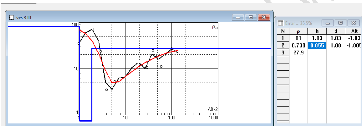
Fig.8:VES station 3 showing graph of apparent resistivity against electrode spacing.
