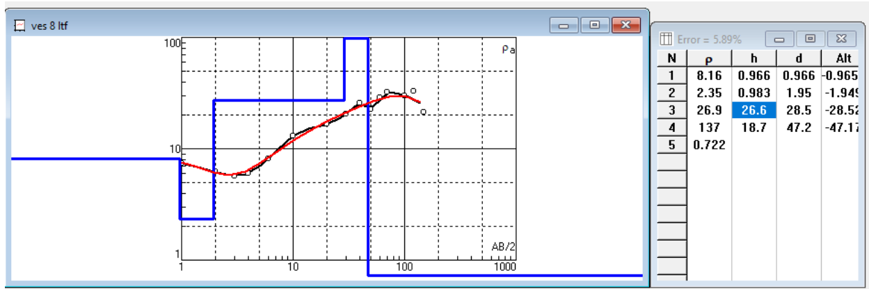
Fig.13: VES station 8 showing graph of apparent resistivity against electrode spacing.
