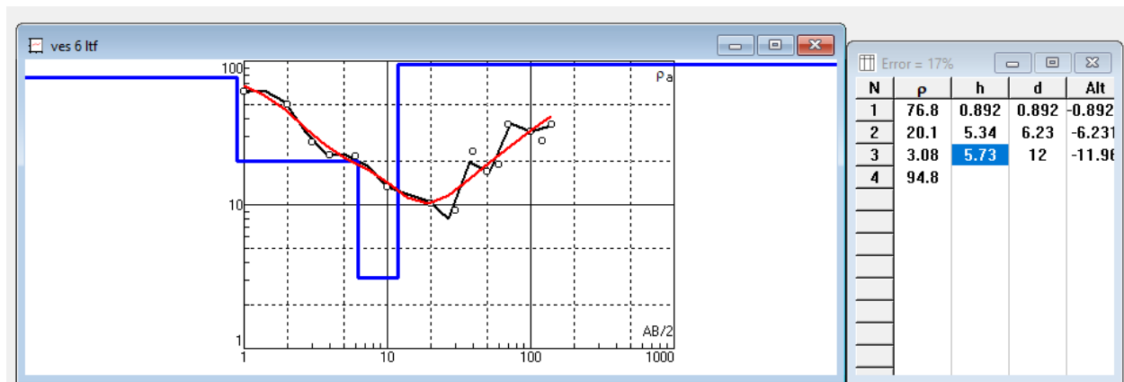
Figure 11: VES station 6 showing graph of apparent resistivity against electrode spacing.
