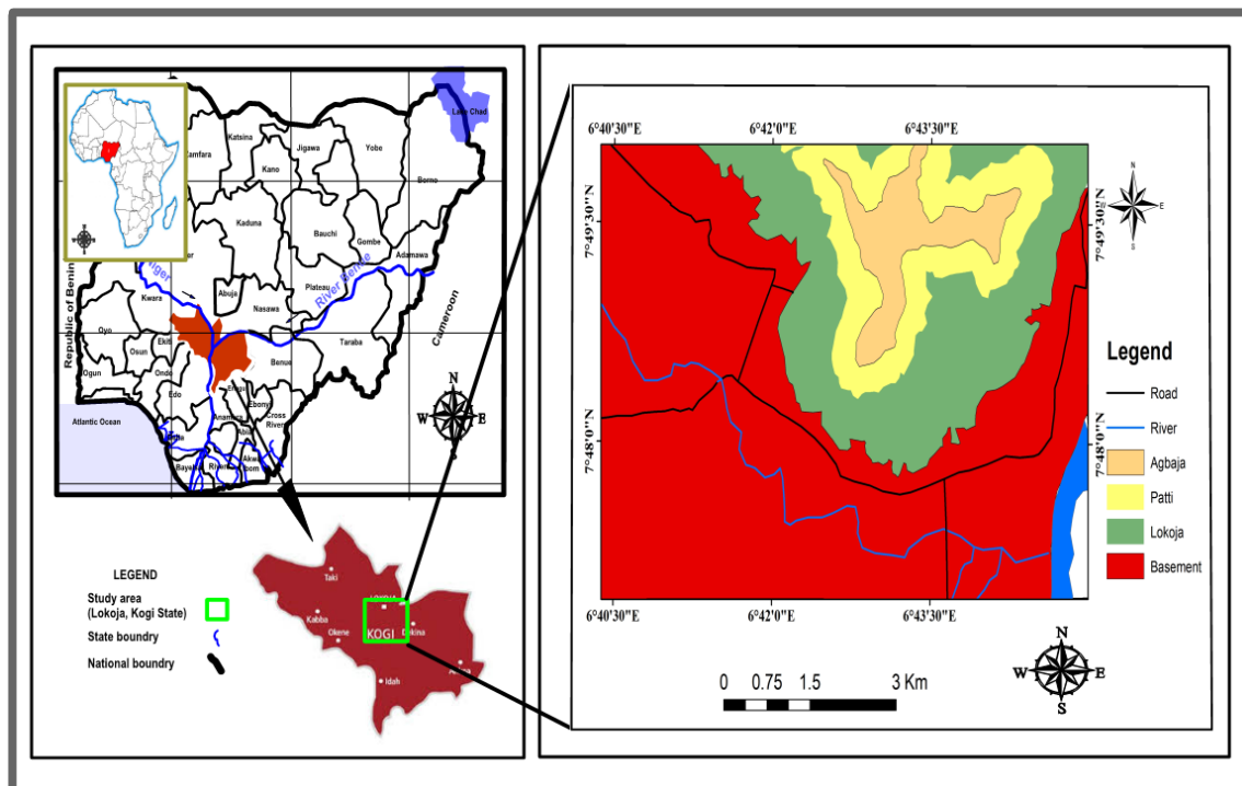
Fig.:2 Geological map of the study area showing different geology (Modified after Ibrahim et al ; Aminu et al. ,2022a)
