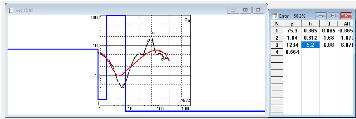
Figure 20: VES station 15 showing graph of apparent resistivity against electrode spacing.
