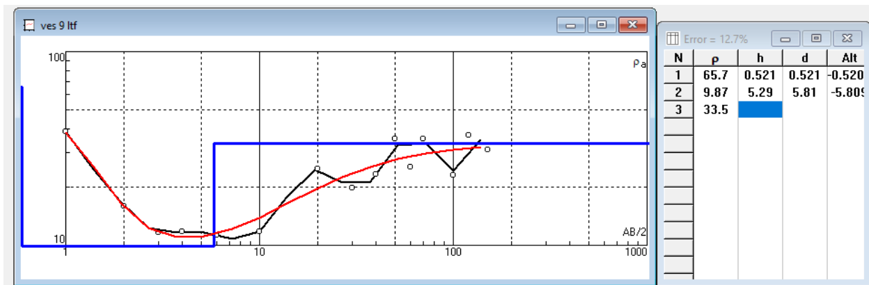
Figure 14: VES station 9 showing graph of apparent resistivity against electrode spacing.
