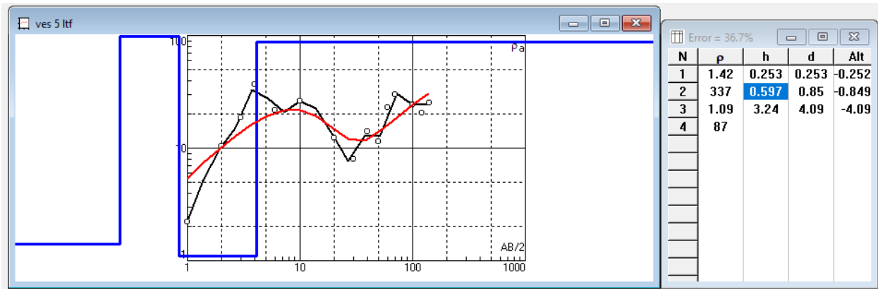
Figure 10: VES station 5 showing graph of apparent resistivity against electrode spacing.
