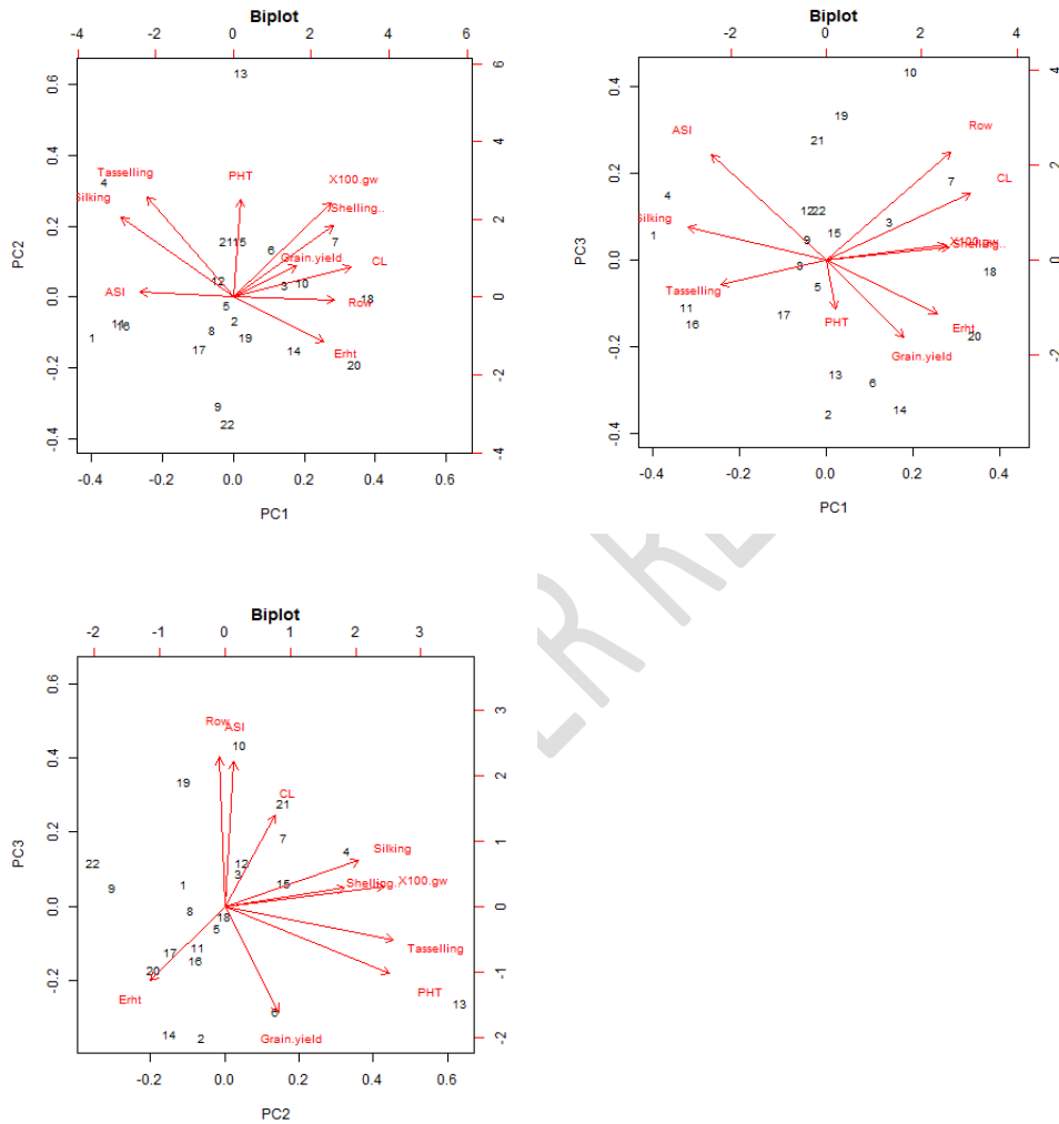
Fig. 2. Principal Component Analysis – Biplot (irrigated condition)
