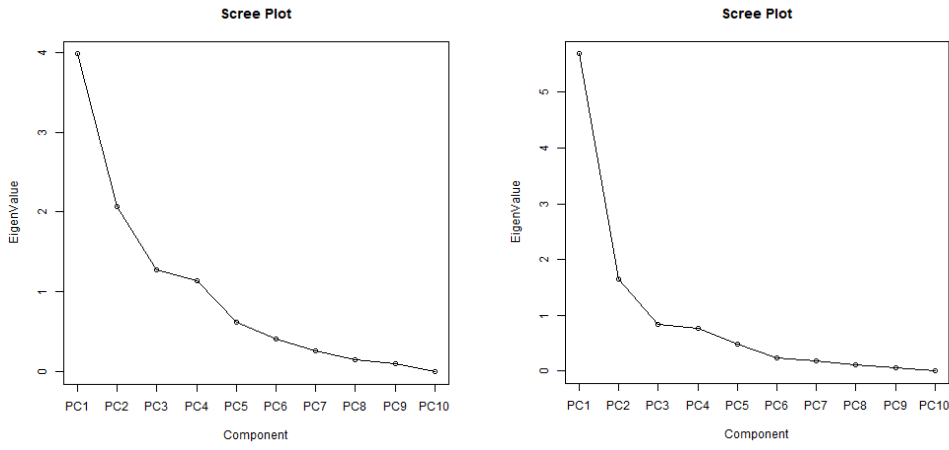
Fig. 1. Scree plot under irrigated and rainfed conditions
