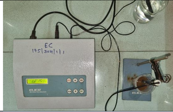
Fig. 4 Indirect measurement of soil salinity using EC meter
