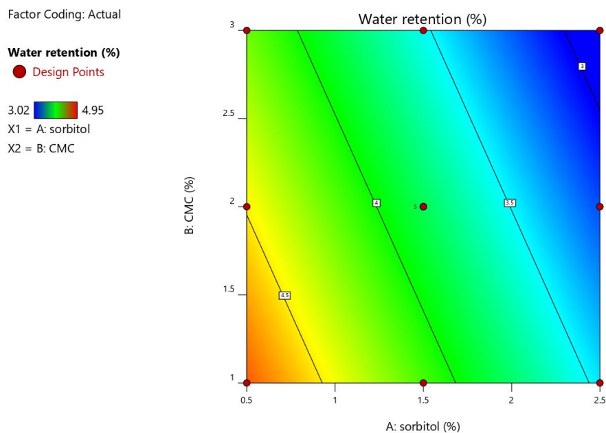
Fig. 1: Contour of interaction effect of CMC and sorbitol concentrations on the water retention of the deep fat fried plantain strips.
