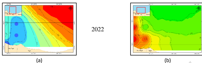
Fig 4. Spatial distribution of Sea Surface Temperature (a) Spatial distribution of Chlorophyll-a (b)
