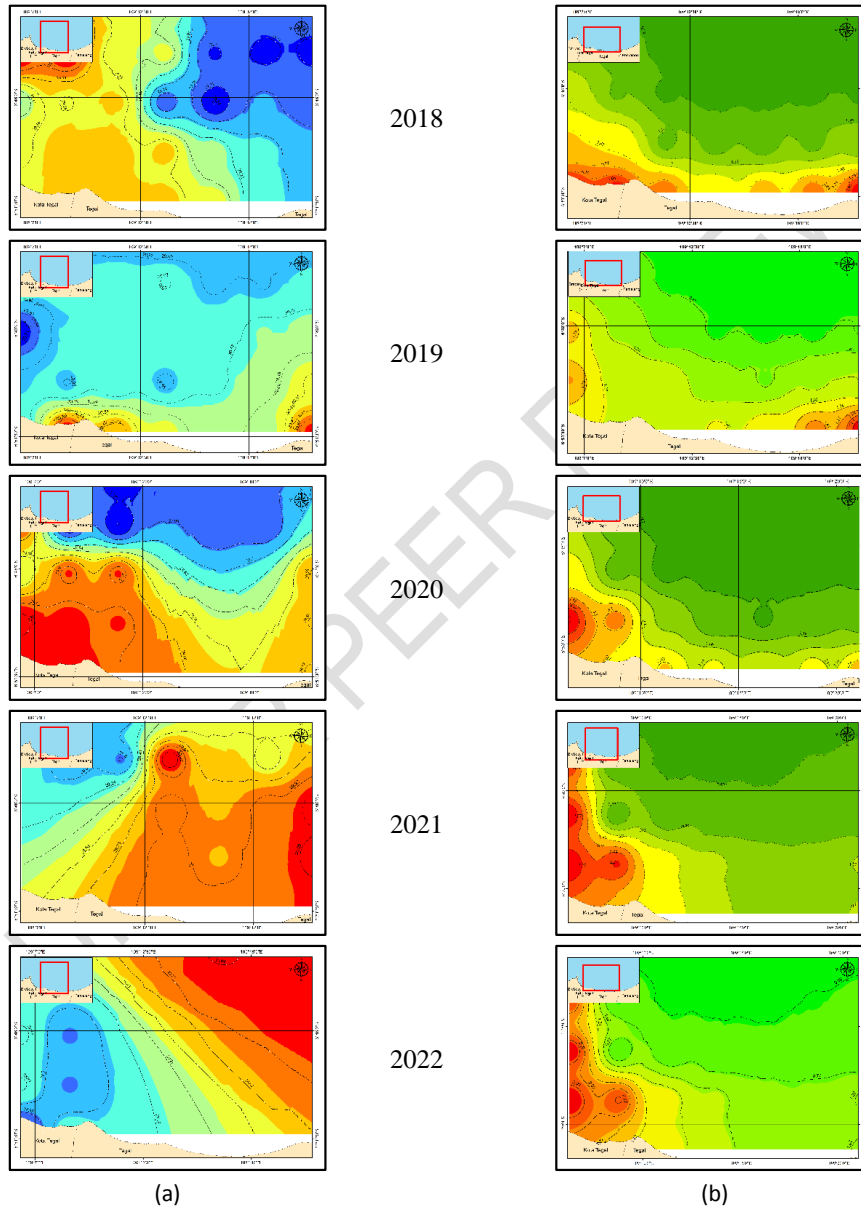
Fig 4. Spatial distribution of Sea Surface Temperature (a)
