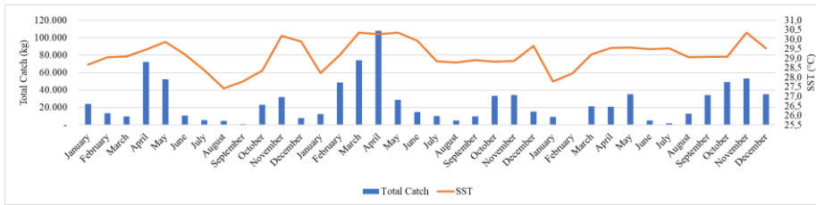
Fig 2. Graph of SST Relationship to Catch
