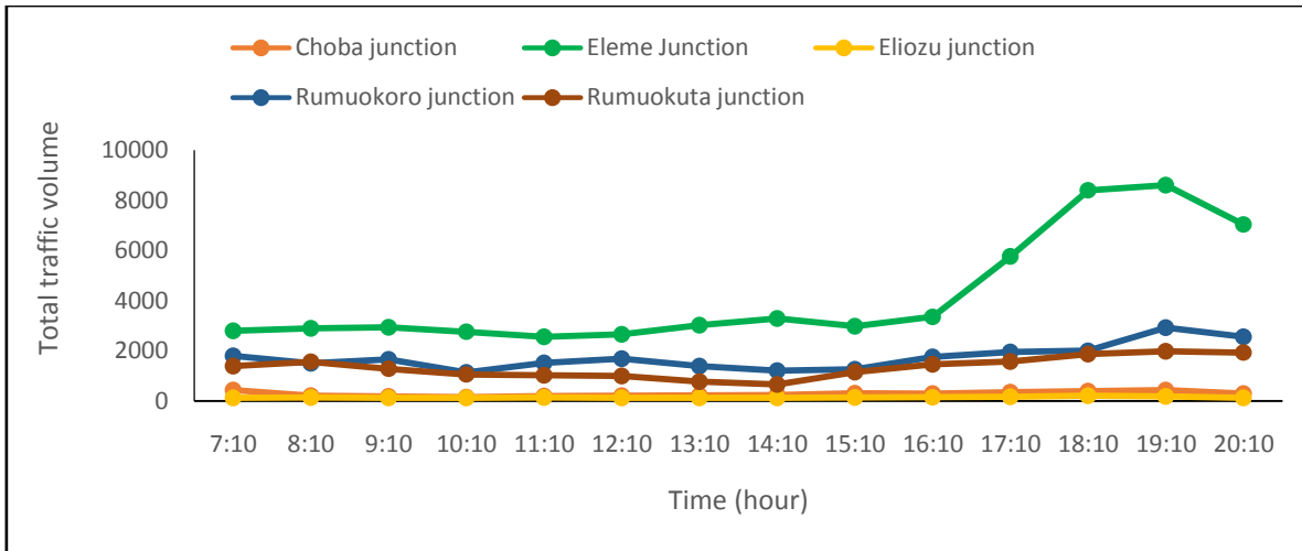
Figure 2: Traffic variations with time
