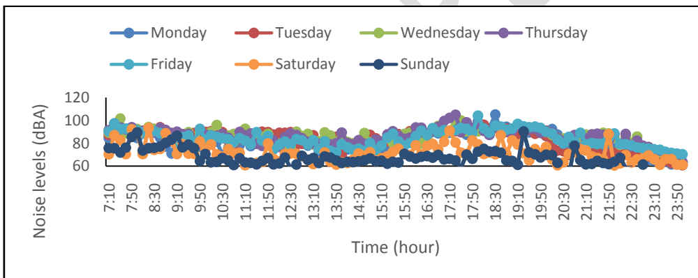
Figure 5: Daily variations of noise levels at Elioazu junction
