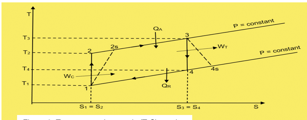
Figure 3: Temperature-Isentropic (T-S) graph
