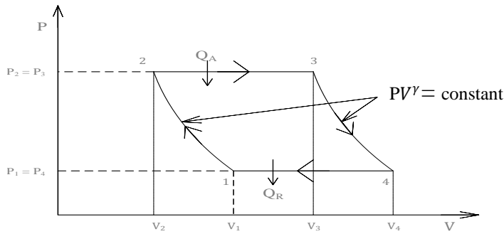
Figure 2: Pressure-volume (P-V) graph
