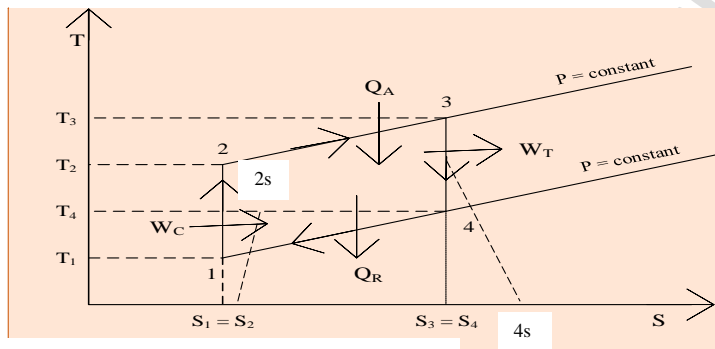
Figure 3: Temperature-Isentropic (T-S) graph
