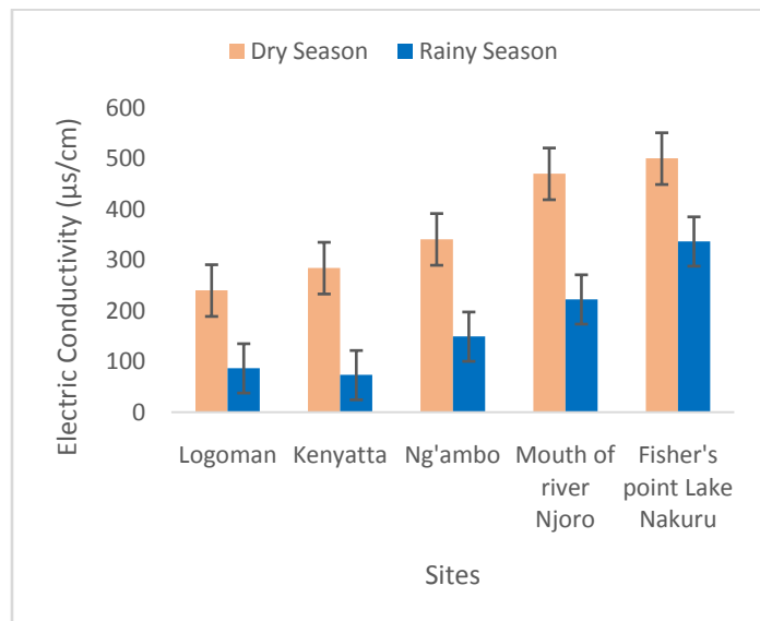
Figure 2: Mean \pm SE variations in conductivity for river Njoro and Lake Nakuru sample points
