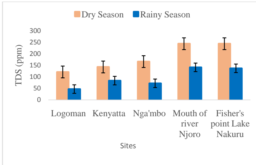
Figure 6: Mean \pm SE TDS for River Njoro and Lake Nakuru sample points
