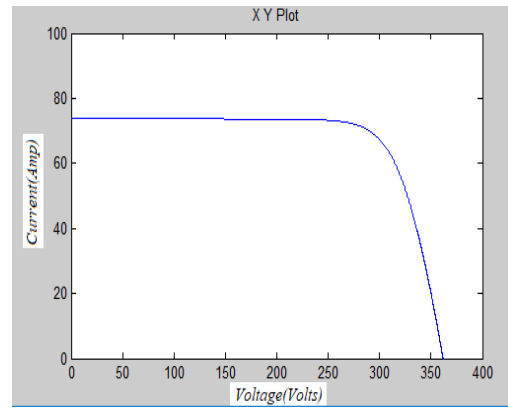
Fig.1: P-V Curve of the PV Module
