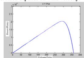
Fig5; I-V curve of PV Module.
