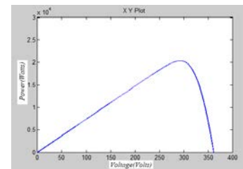
Fig4; I-V curve of PV Module.
