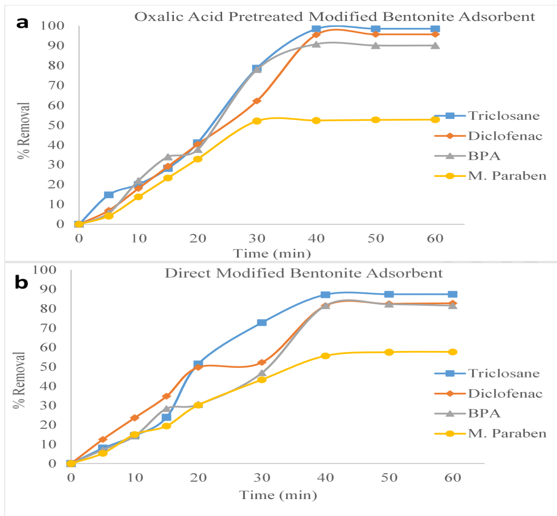
Fig7 Effect of contact time on ECs removal (a) Oxalic acid pretreated and (b) Direct organo-modified bentonite adsorbent
