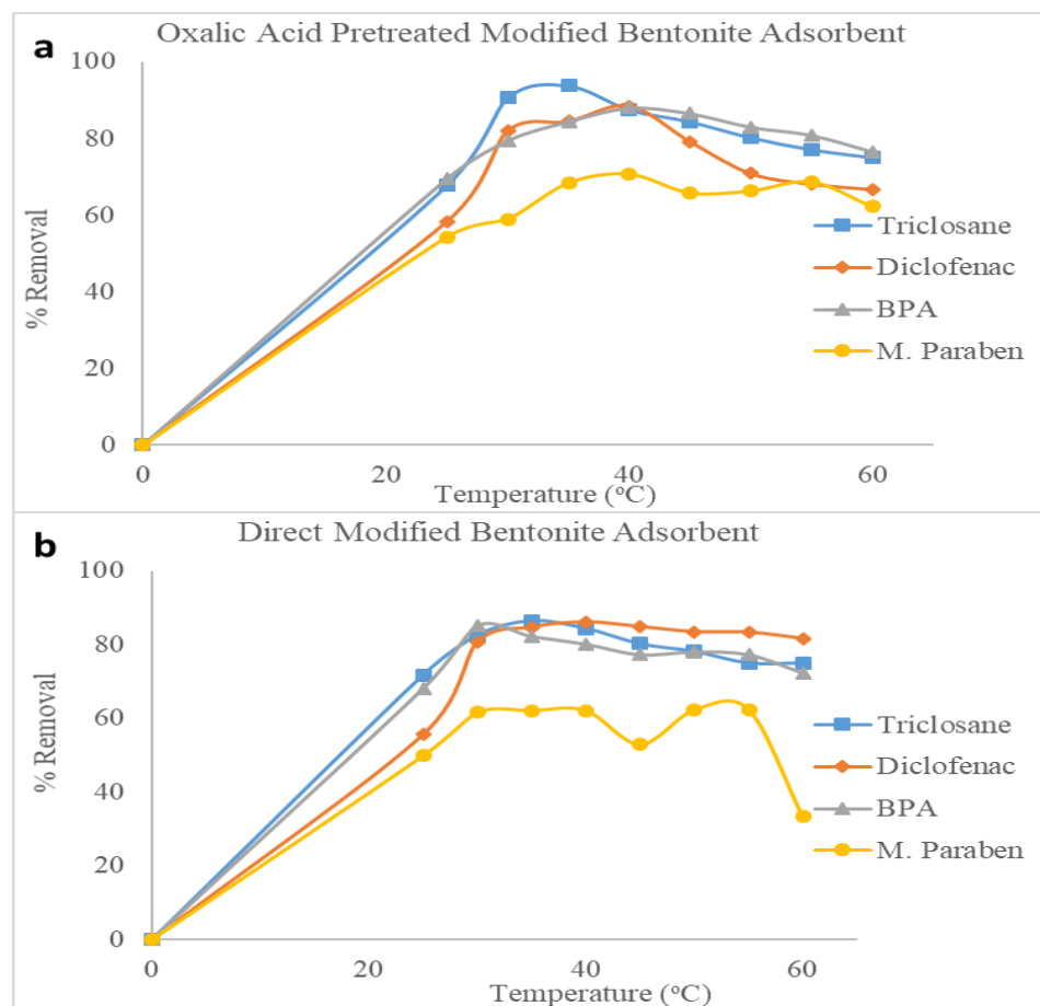
Fig 9 Effect of temperature on ECs removal (a) Oxalic acid pretreated and (b) Direct organo-modified bentonite adsorbent
