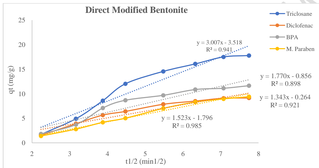
Fig 11 Intraparticle diffusion model for the adsorption of ECs into direct MB
