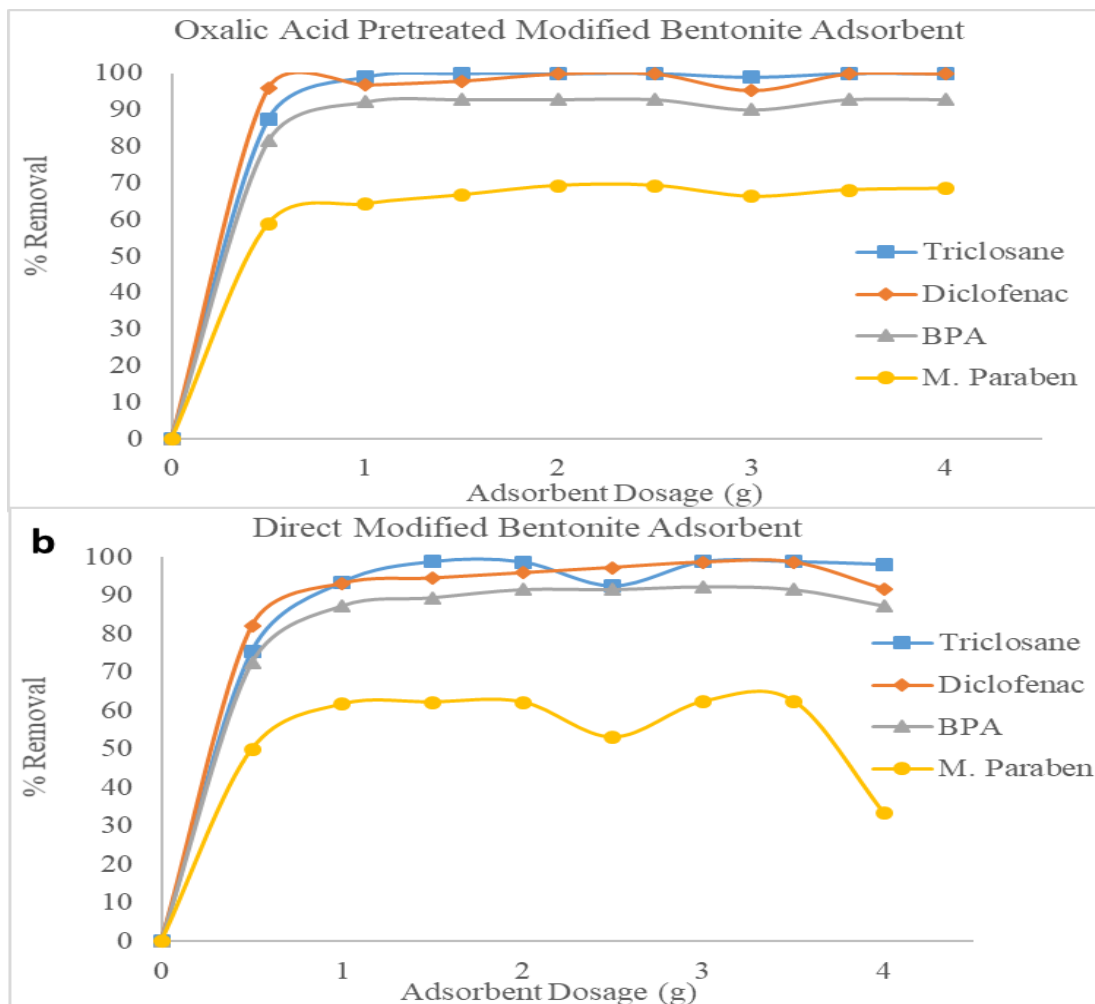
Fig 8 Effect of adsorbent dosage on ECs removal (a) Oxalic acid pretreated and (b) Direct organo-modified bentonite adsorbent
