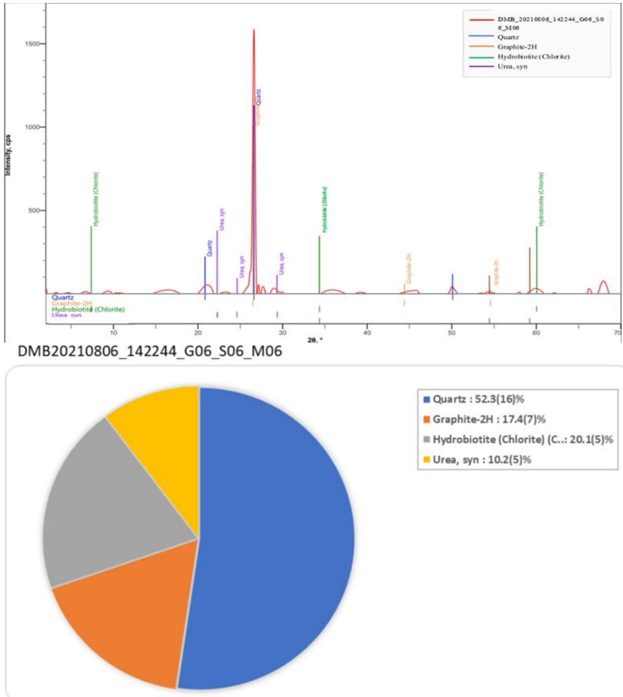
Fig 3 XRD pattern of modified bentonite (DMB) adsorbent before adsorption
