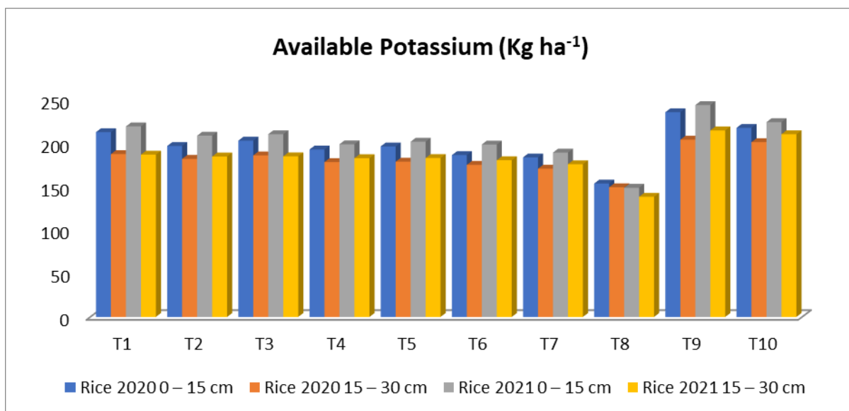
Fig. 6 Impact of crop residue and green manure on soil available potassium
