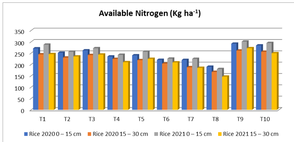
Fig. 4 Impact of crop residue and green manure on soil available nitrogen
