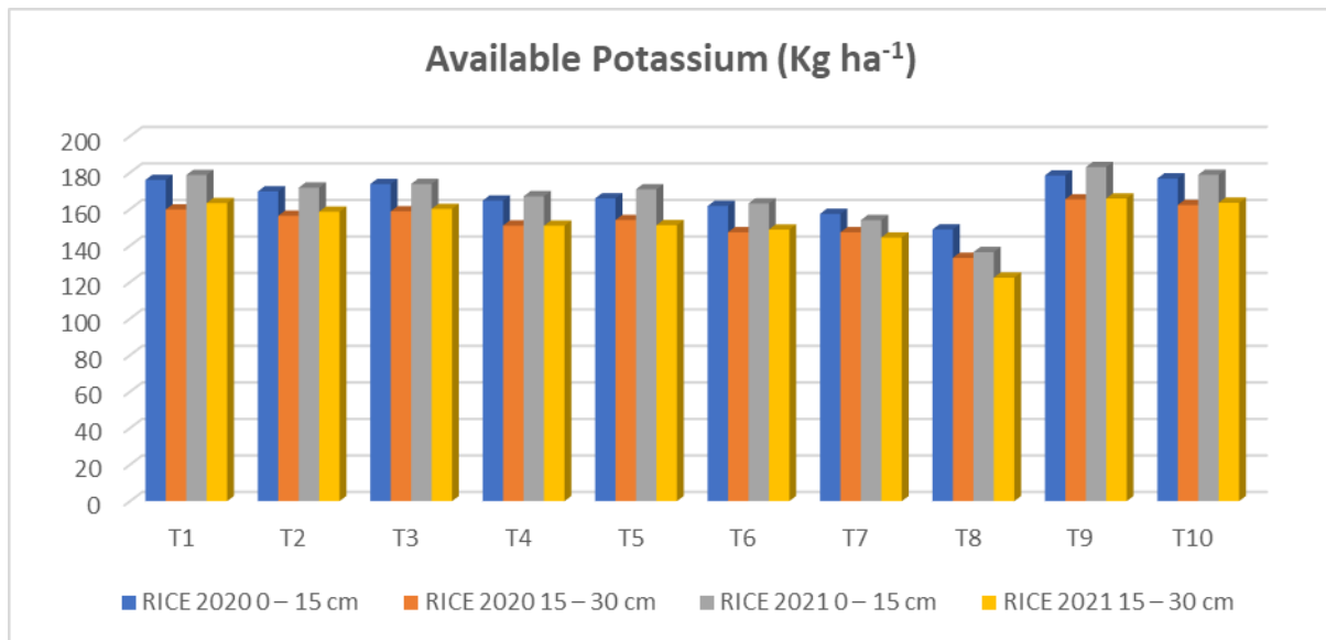
Fig. 5 Impact of crop residue and green manure on soil available phosphorus
