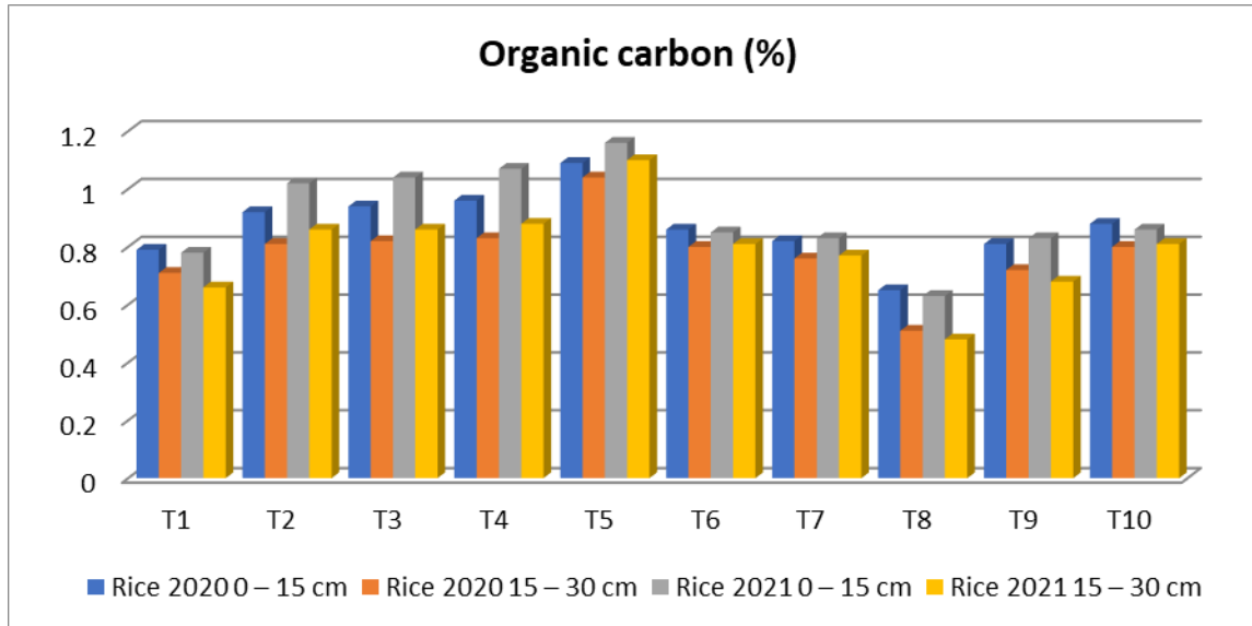
Fig. 3 Impact of crop residue and green manure on soil organic carbon
