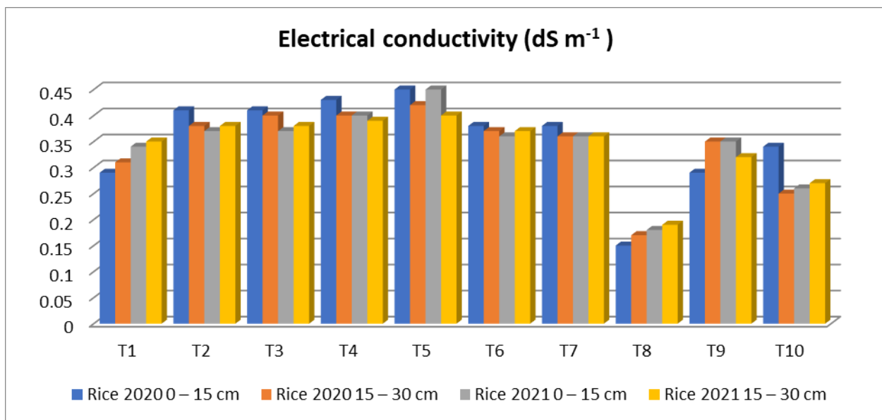
Fig. 2 Impact of crop residue and green manure on soil EC
