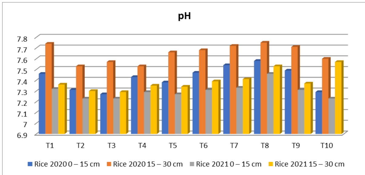
Fig. 1 Impact of crop residue and green manure on soil pH
