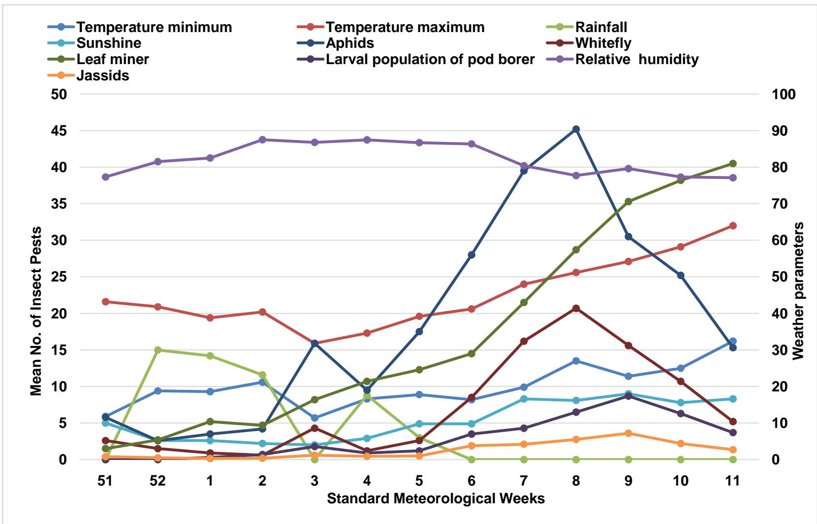
Fig. 1: Incidence of pest spectra in French bean under the influence of weather factors during Rabi 2021-22.
