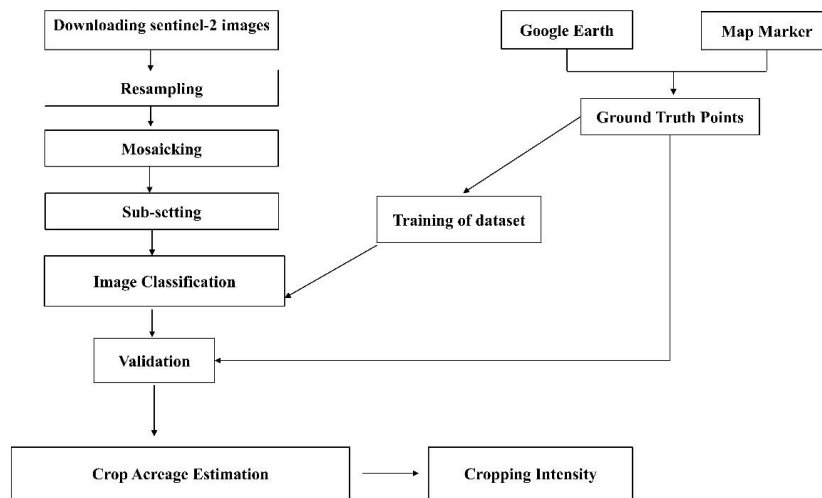
Fig. 2. The flowchart of the methodology followed
