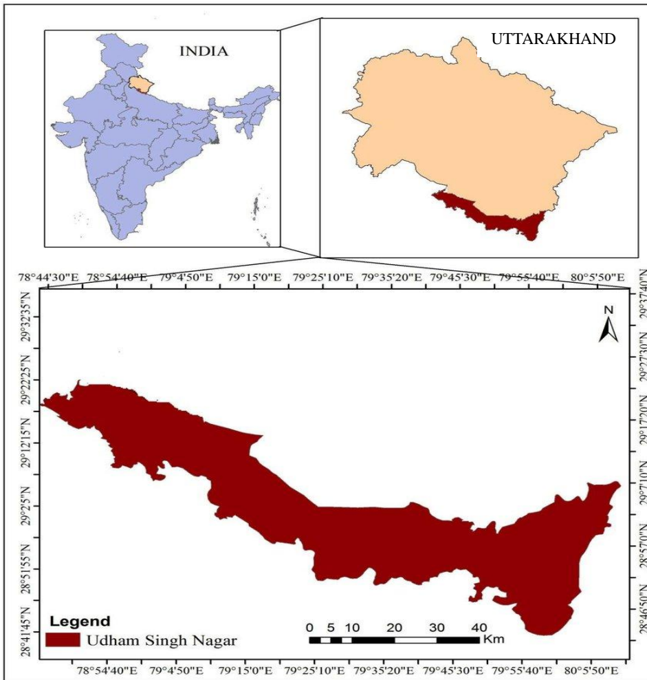
Fig. 1. Location map of Udham Singh Nagar district
