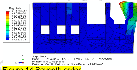
Figure 14 Seventh order
