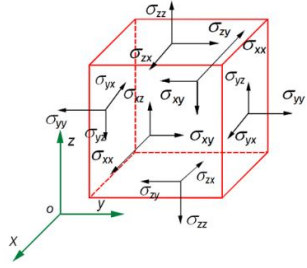
Figure 3 Differential Unit Body
