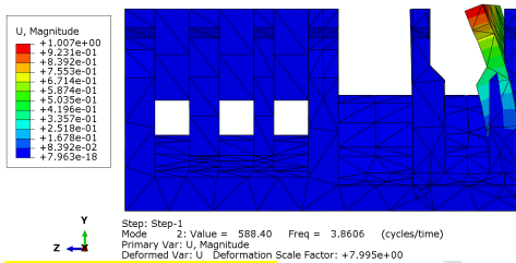
Figure 9 Second order
