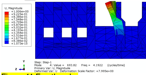
Figure 11 Fourth order
