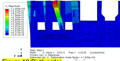
Figure 13 Sixth order
