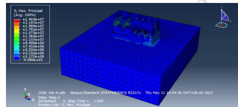
Figure 6 Cloud Chart of the First Principal Stress of the Dam
