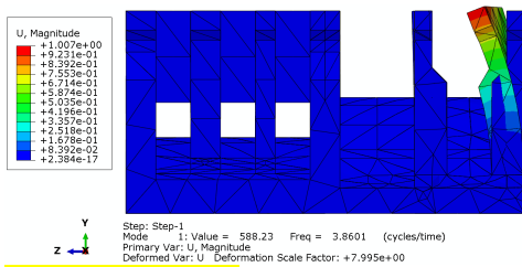
Figure 8 First order
