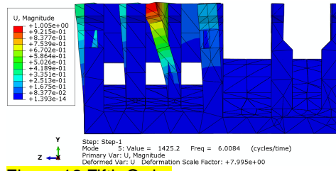
Figure 12 Fifth Order
