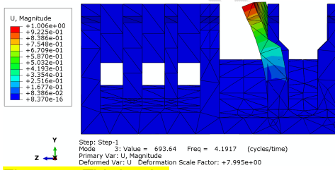
Figure 10 Third order
