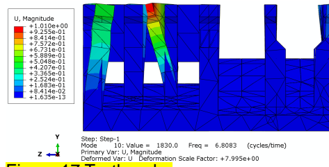
Figure 17 Tenth order
