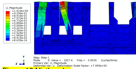
Figure 16 Ninth order
