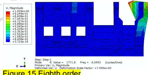
Figure 15 Eighth order
