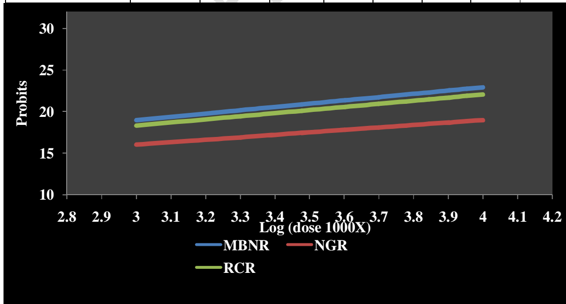
Fig. 3: Log dose probit lines of spinosad against the three populations of H. armigera (MBNR – Mahaboobnagar, NGR – Nagpur, RCR – Raichur)
