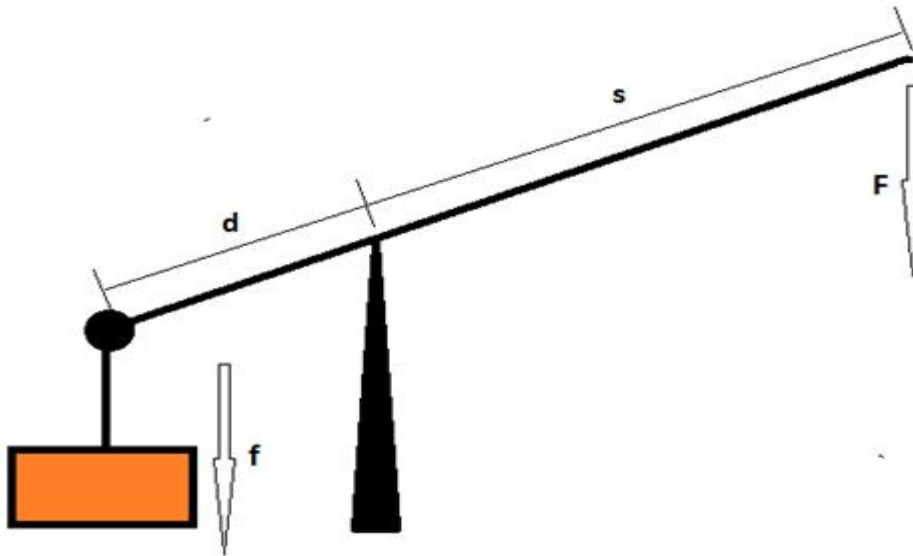
Figure: d=1\text{ m} , s= 3\text{ m} , f is the weight of the block =60\text{ kgf} , F =20\text{ kgf} , F*s=f*d
