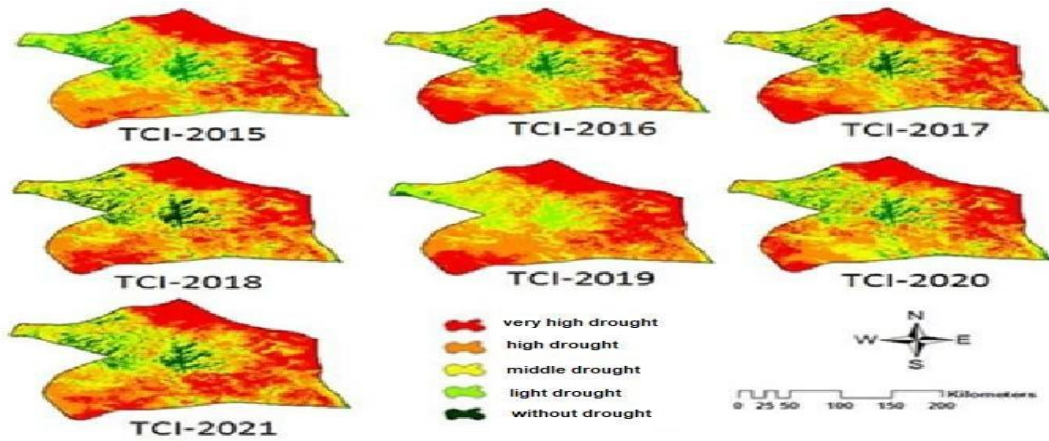
Figure .5 Temperature Condition Index during (TCI) 2015 – 2021
