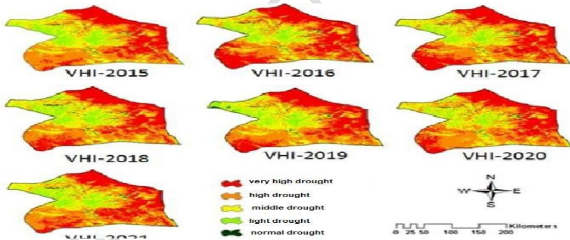
Figure 6.vegetation health index (VHI) during 2015-2021
