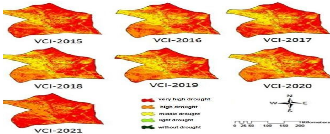
Figure 7.vegetation condition index (VCI) during 2015-2021
