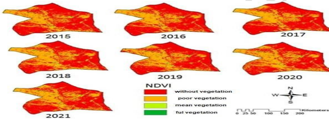
Figure.4 the normalized difference vegetation index (NDVI) during 2015 – 2021
