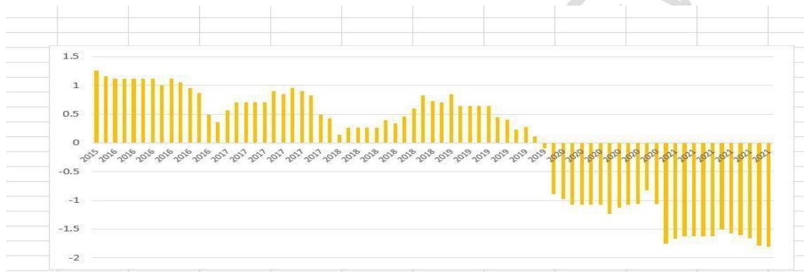
Figure3.Monthly average of synoptic station data during 2015 – 2021(mm)
