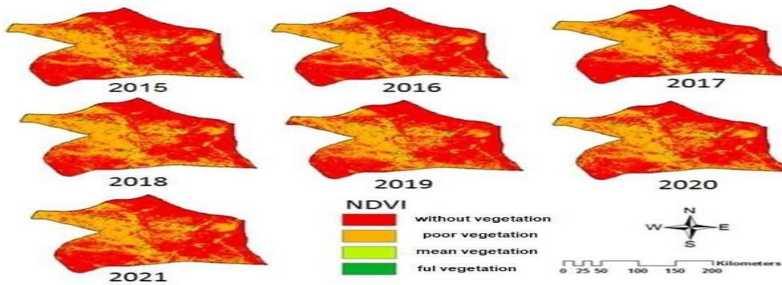
Figure.4 the normalized deference vegetation index (NDVI) during 2015 – 2021
