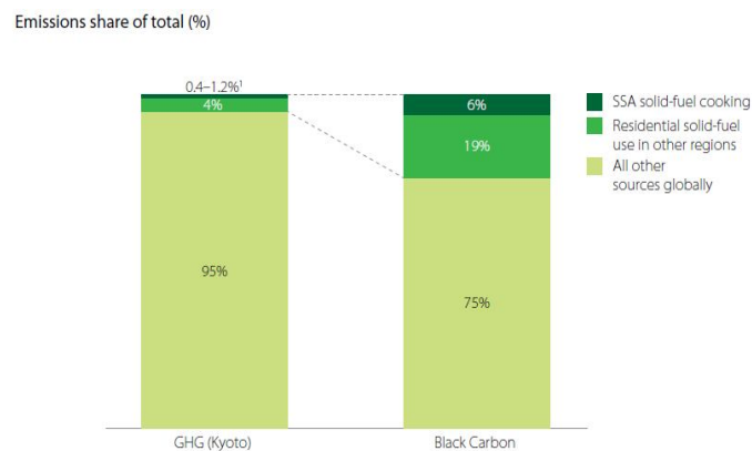
Figure 1-8 Black carbon and GHG emissions from solid-fuel cooking in SSA (The World Bank, 2014)
