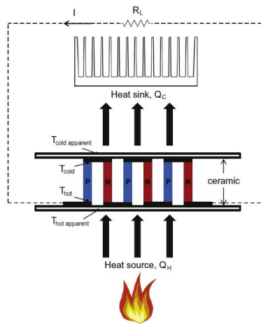
Figure 1-10 Thermoelectric Power Generation (O'Shaughnessy, et al., 2012)
