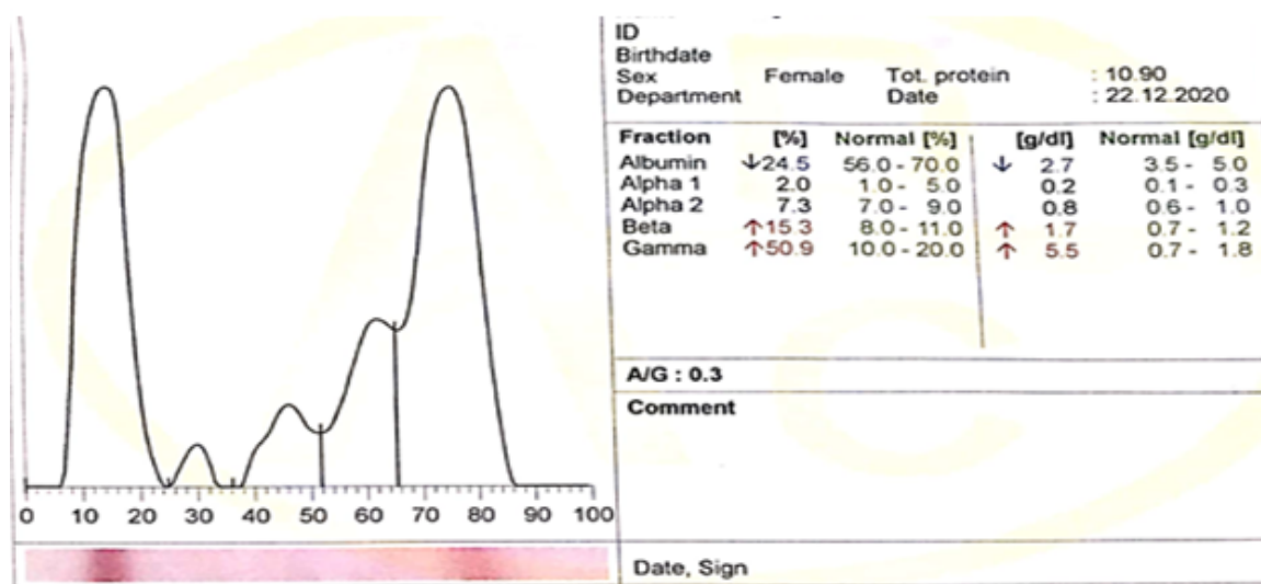
Figure 1 Serum Protein electrophoresis of patient 65 years ; Albumin= 24%, Alpha1= 2.0 %, Alpha 2= 7.3% , Beta 1= 15.3% , Gamma Globulin= 50.9 %.
