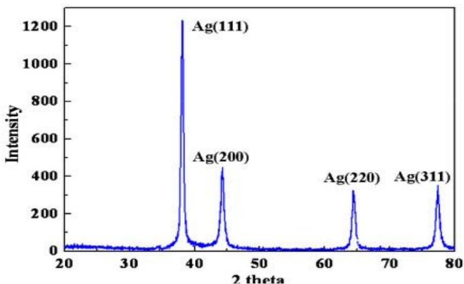
Fig. 3. X-ray diffraction pattern of silver nanoparticles
