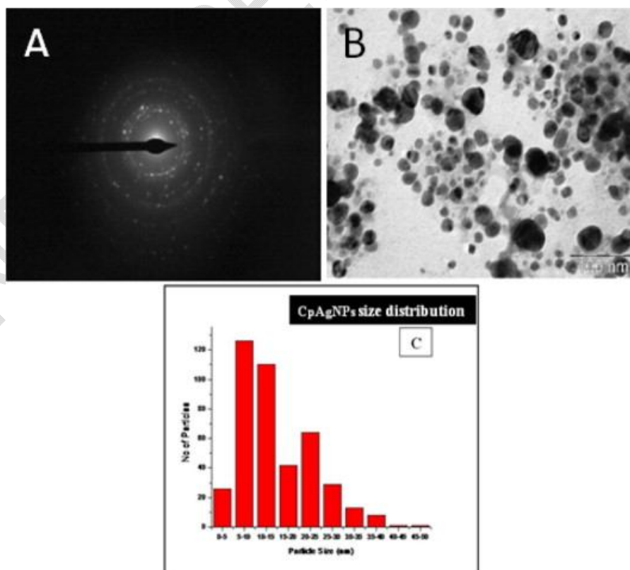
Figure 6: Transmission electron microscope images silver nanoparticles
