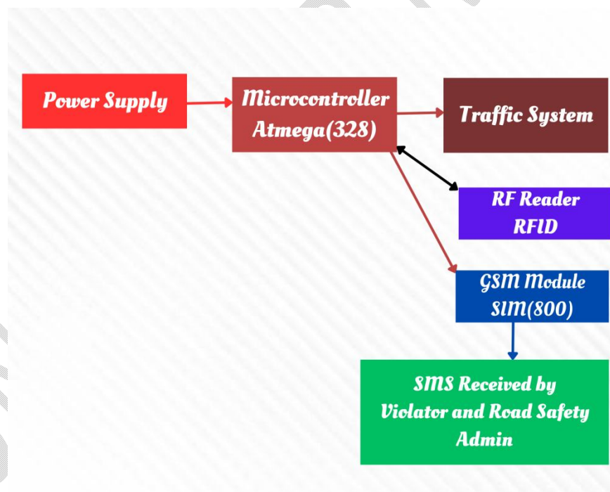
Figure. 1. Block Diagram of an Automated Ticketing System
