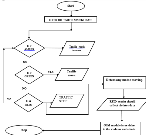
Figure. 4. System Flowchart
