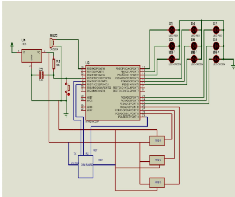
Figure. 3. The Circuit Diagram of an Automated Ticketing System using Radio Frequency Identification (RFID)
