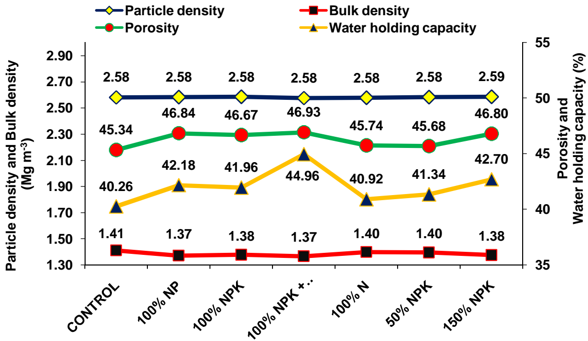
Figure 1. Trend of physical properties under different long-term nutrient management practices across 0-60 cm soil depth.
