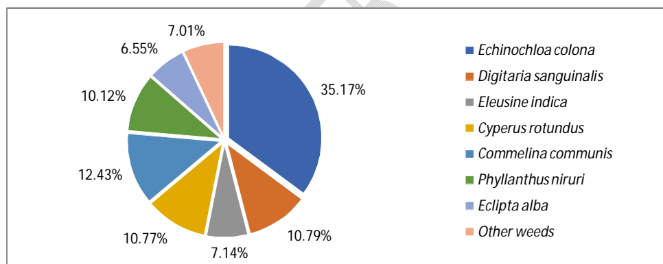
Figure 1. Relative density of weeds at 30 and 45 DAS
