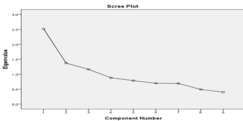
Figure 10: Scree plot
