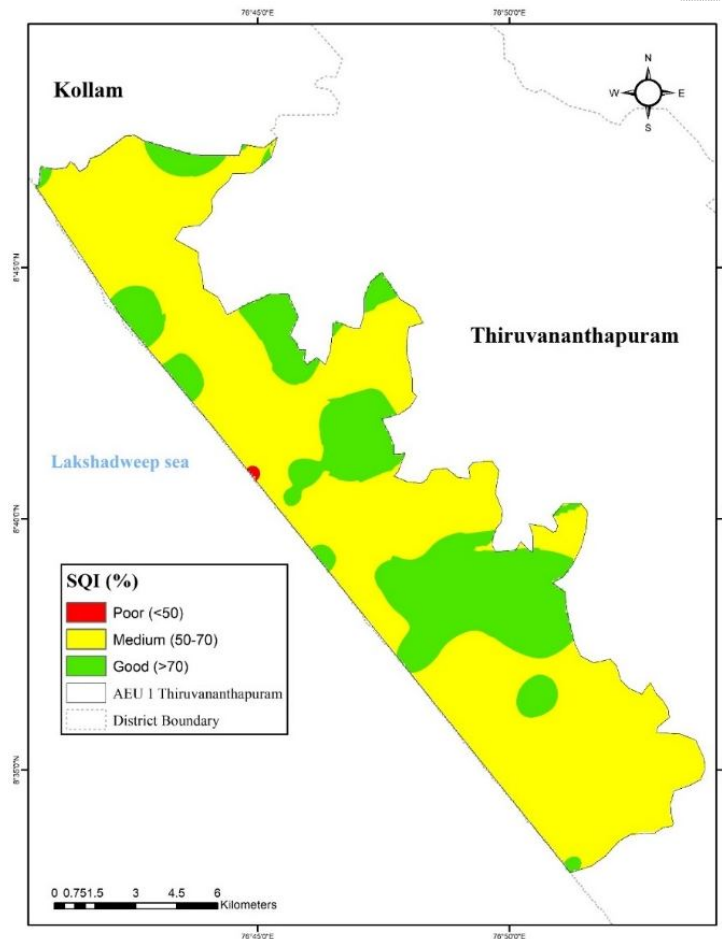
Fig. 4. Spatial variability of RSQI in AEU 1, Thiruvananthapuram district
