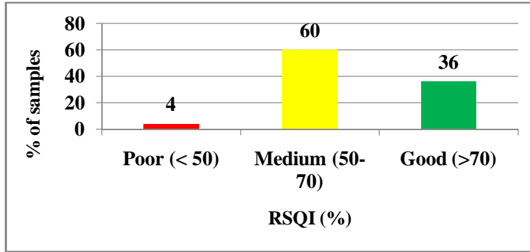
Fig. 3. Frequency distribution of relative soil quality index in the soils of AEU 1
