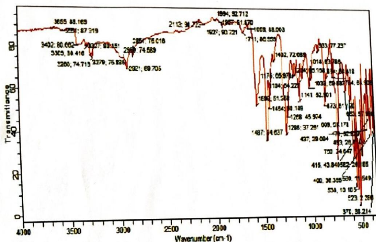
Figure 1: FTIR of Cobalt (II) complex
