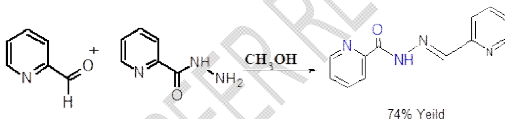
N' -[( E )-(pyridin-2-yl)methylidene]pyridine-2-carbohydrazide
