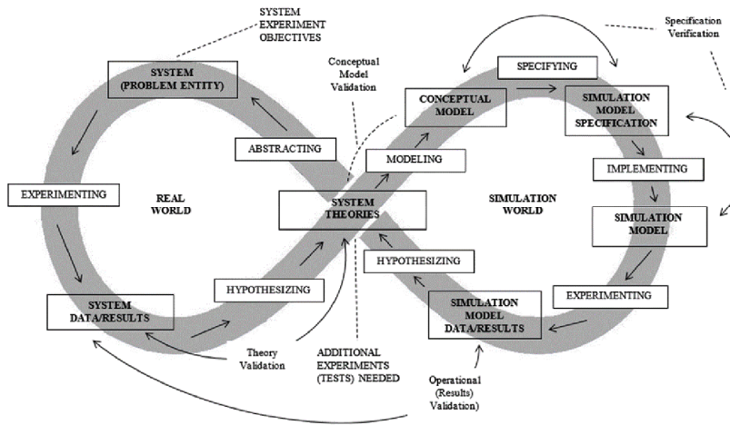
Fig. 3. Stages of problem modeling through computer simulation [adapted from (Schriber et al., 2013)].
