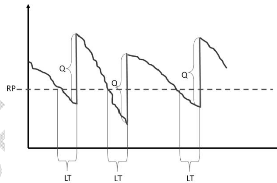
Fig. 2. Parameters and inventory supply/consumption pattern under the continuous review (Q, R) model (Sánchez-Vega et al., 2019).
