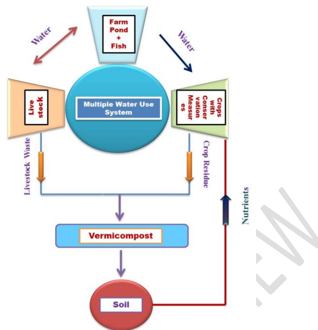
Fig 3. Schematic representation of Multiple water use based IFS
