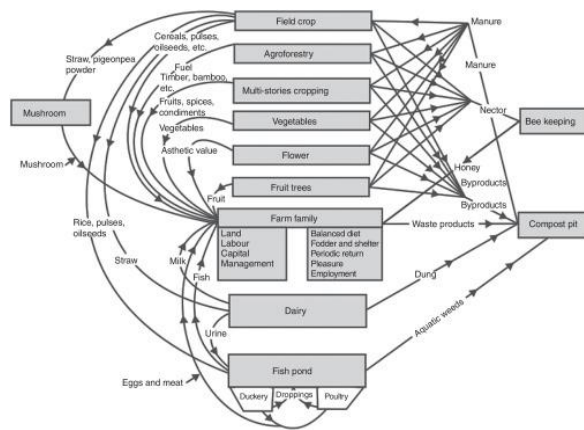
Fig 1. Interactions among different components of an IFS.
