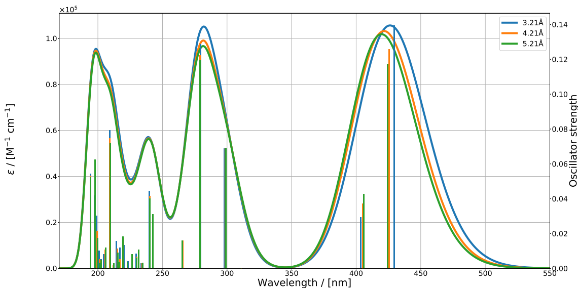
Figure 8: The UV/Vis spectra of s-cis -VHF in the CN orientation with a molecule cluster separation of 3.21 Å, 4.21 Å, and 5.21 Å, respectively. The extinction coefficient/the molar absorptivity is denoted by \epsilon .
