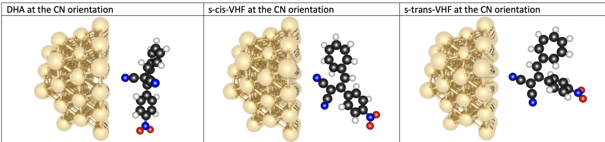
Figure 6: The CN orientation of DHA, s-cis-VHF, and s-trans-VHF, respectively. The extinction coefficient/the molar absorptivity is denoted by \epsilon .
