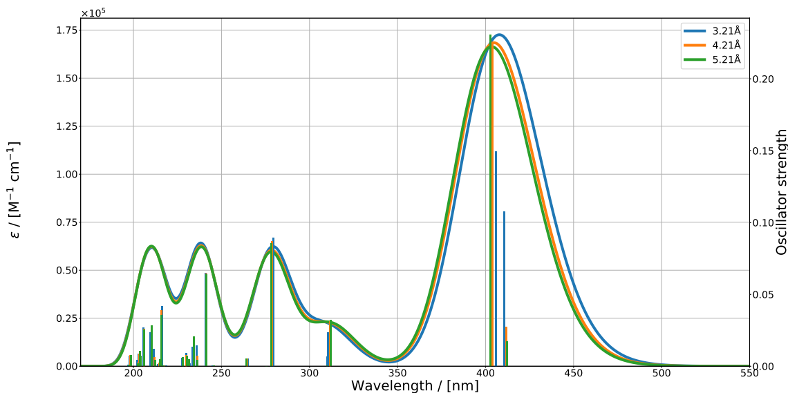
Figure 9: The UV/Vis spectra of s-trans -VHF in the CN orientation with a molecule cluster separation of 3.21 Å, 4.21 Å, and 5.21 Å, respectively. The extinction coefficient/the molar absorptivity is denoted by \epsilon .
