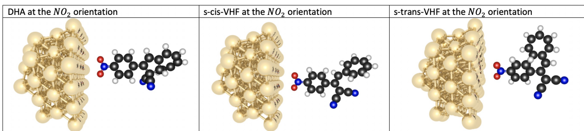
Figure 2: The \text{NO}_2 orientation of DHA, s-cis -VHF, and s-trans -VHF respectively.
