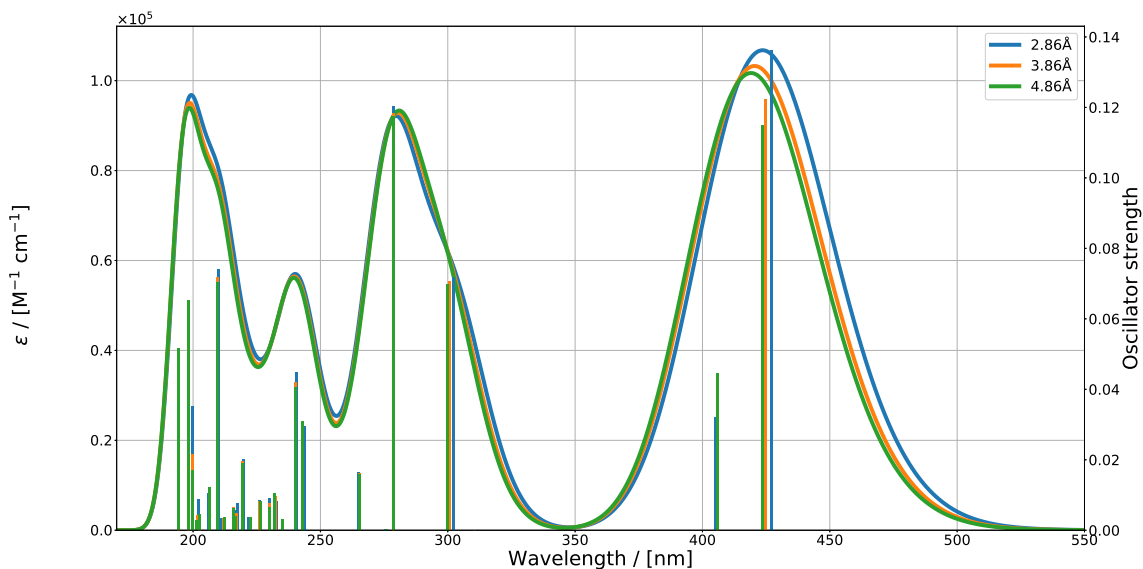
Figure 12: The UV/Vis spectra of s-cis -VHF in the 7mem orientation with a molecule cluster separation of 2.86 Å, 3.86 Å, and 4.86 Å, respectively. The extinction coefficient/the molar absorptivity is denoted by \epsilon .
