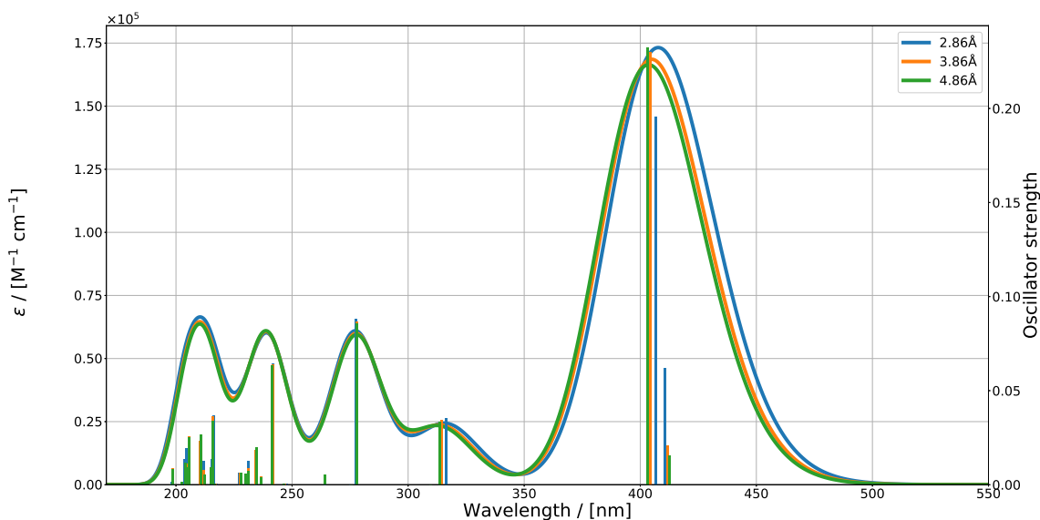
Figure 13: The UV/Vis spectra of s-trans -VHF in the 7mem orientation with a molecule cluster separation of 2.86 Å, 3.86 Å, and 4.86 Å, respectively. The extinction coefficient/the molar absorptivity is denoted by \epsilon .
