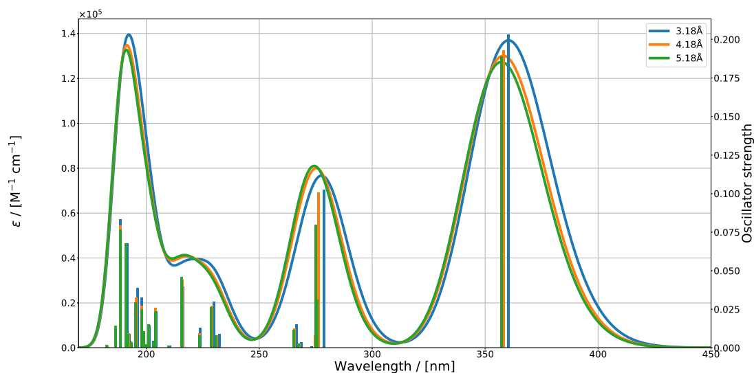
Figure 3: The UV/Vis spectra of DHA in the \text{NO}_2 orientation with a molecule cluster separation of 3.18 Å, 4.18 Å, and 5.18 Å, respectively. The extinction coefficient/the molar absorptivity is denoted by \epsilon .
