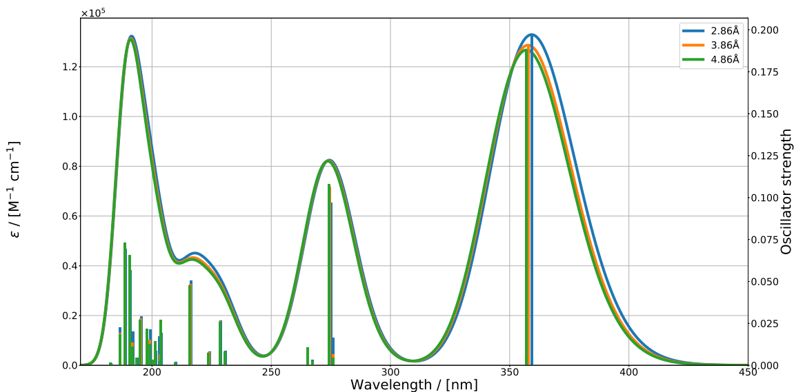
Figure 11: The UV/Vis spectra of DHA in the 7mem orientation with a molecule cluster separation of 2.86 Å, 3.86 Å, and 4.86 Å, respectively. The extinction coefficient/the molar absorptivity is denoted by \epsilon .
