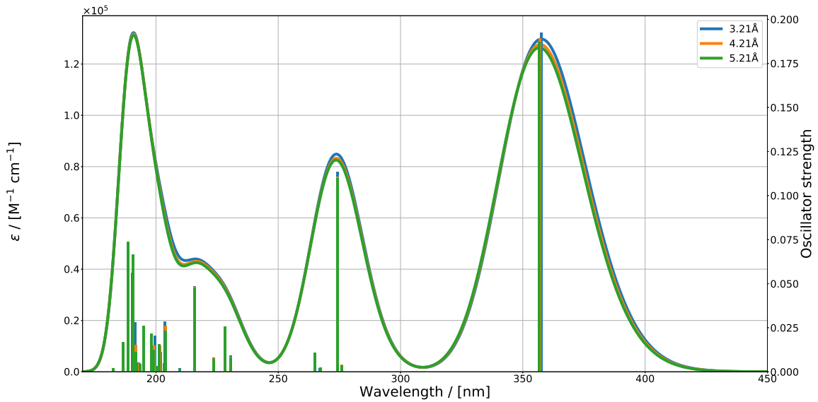
Figure 7: The UV/Vis spectra of DHA in the CN orientation with a molecule cluster separation of 3.21 Å, 4.21 Å, and 5.21 Å, respectively. The extinction coefficient/the molar absorptivity is denoted by \epsilon .
