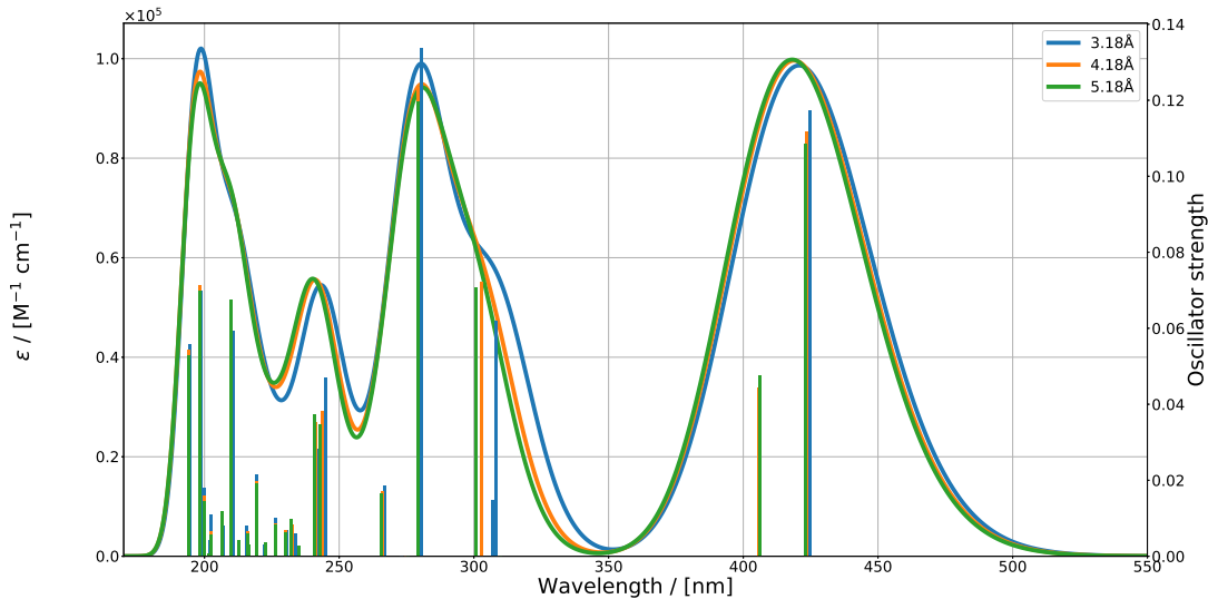
Figure 4: The UV/Vis spectra of s-cis -VHF in the NO_2 orientation with a molecule cluster separation of 3.18 Å, 4.18 Å, and 5.18 Å, respectively. The extinction coefficient/the molar absorptivity is denoted by \epsilon .
