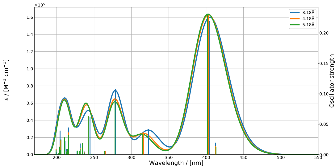
Figure 5: The UV/Vis spectra of s-trans -VHF in the NO_2 orientation with a molecule cluster separation of 3.18 Å, 4.18 Å, and 5.18 Å, respectively. The extinction coefficient/the molar absorptivity is denoted by \epsilon .
