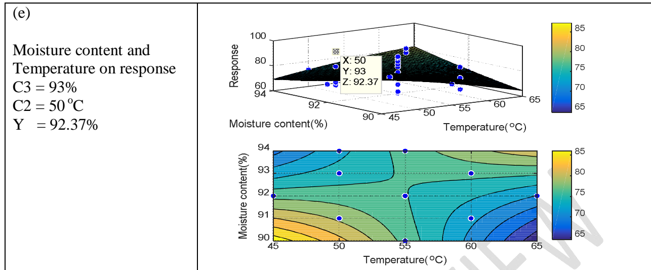
Figure 5: Interaction between input parameters and the response Y (methane yield)
