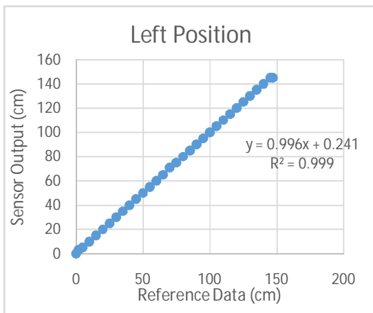
Fig 9. Linear graph of left position tool test data
