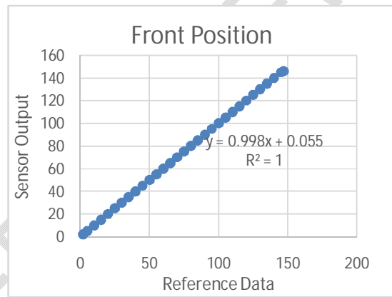
Fig 8. Linear graph of front position tool test data
