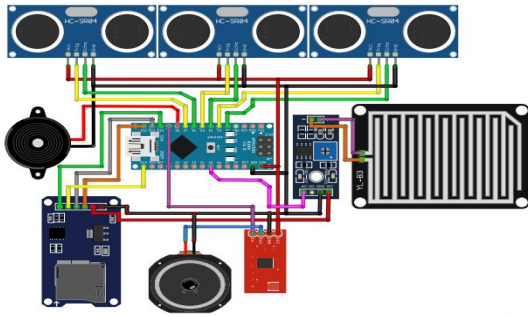
Fig 6. Schematic of all components
