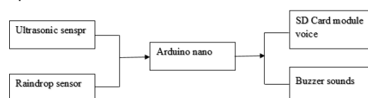
Fig 5. Block diagram of design tool
