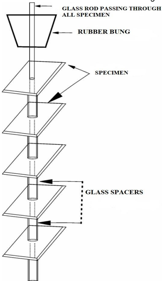
Fig 2: Specimen container
