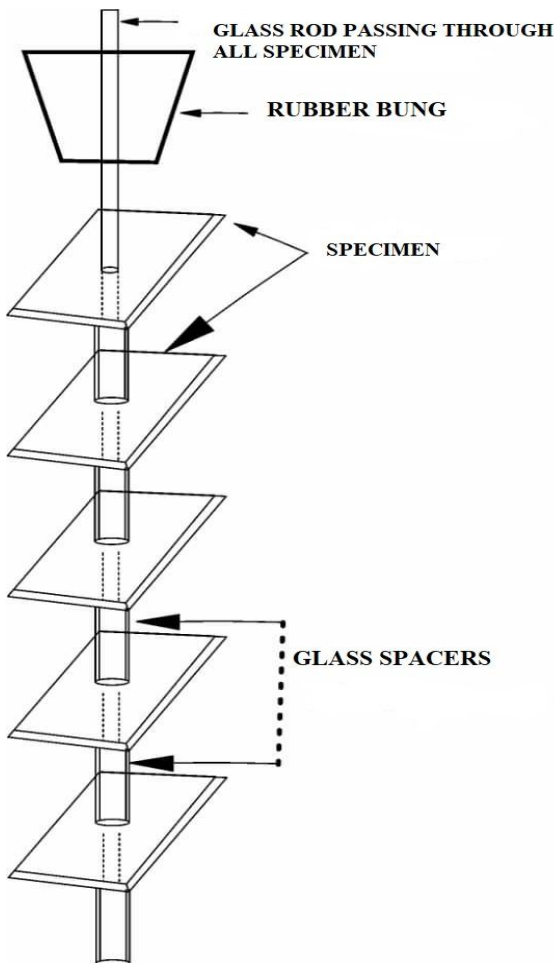
Fig 2: Specimen container
