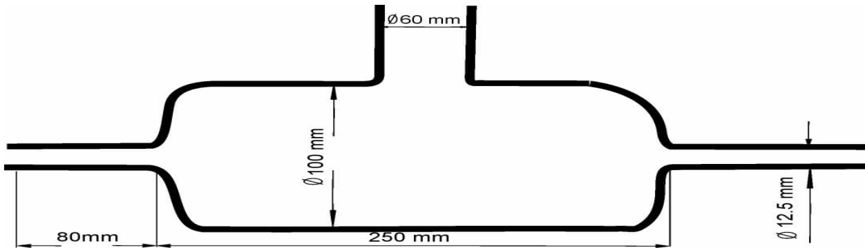
Fig 3: Specimen
