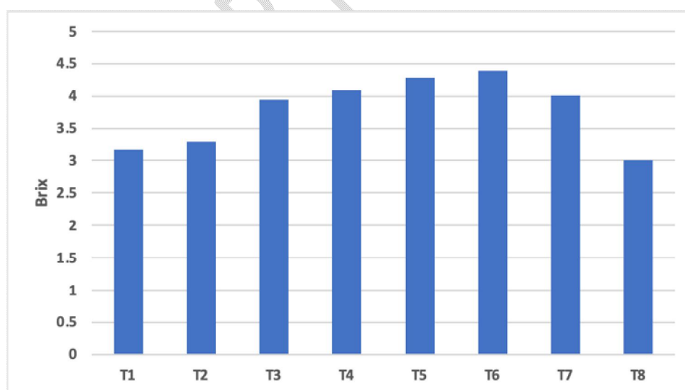
Figure 1. Use of micronutrients and humic acid on TSS (°Brix)
