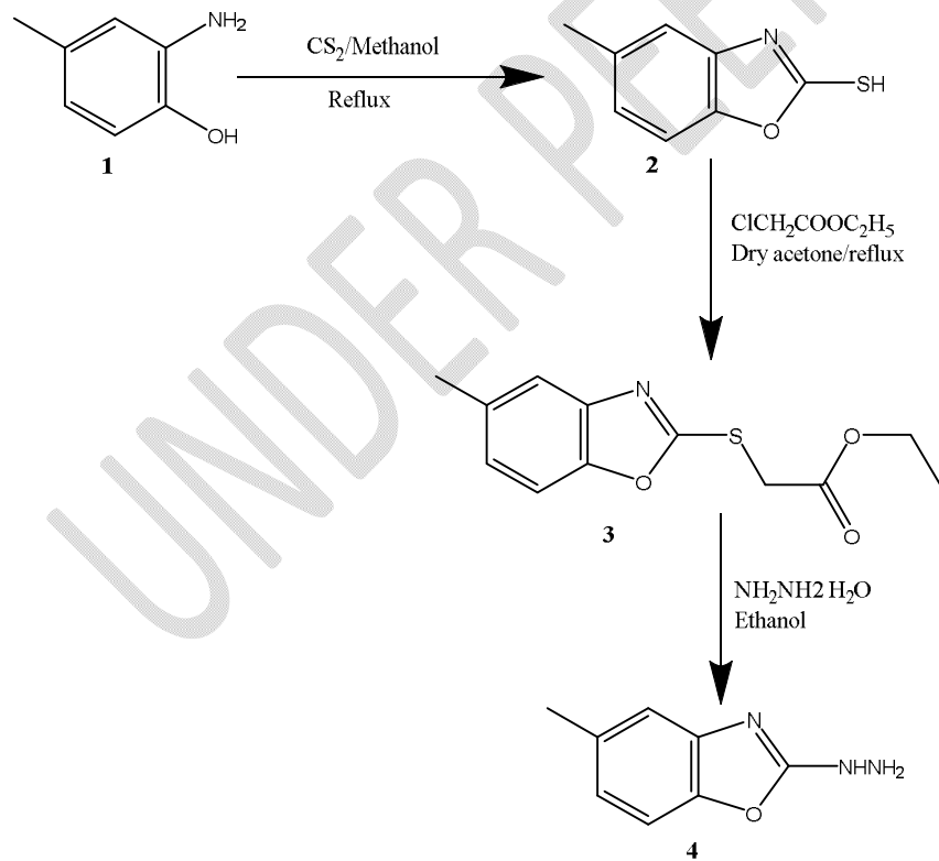
Fig. 5. Synthetic route for the synthesis of Compound 4
