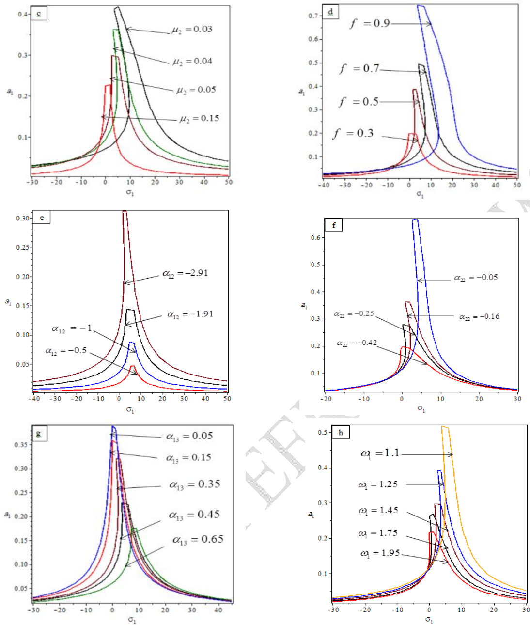
Fig. 4 Effects of different parameters on the detuning parameter ( a_1 against \sigma_1 )
