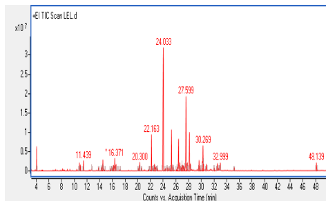
Figure 1: Gas Chromatogram of Lannea egregia leaf essential oil
