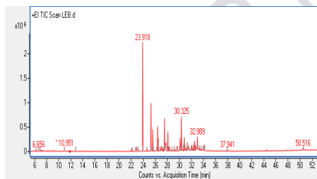
Figure 3: Gas Chromatogram of Lannea egregia stem-bark essential oil
